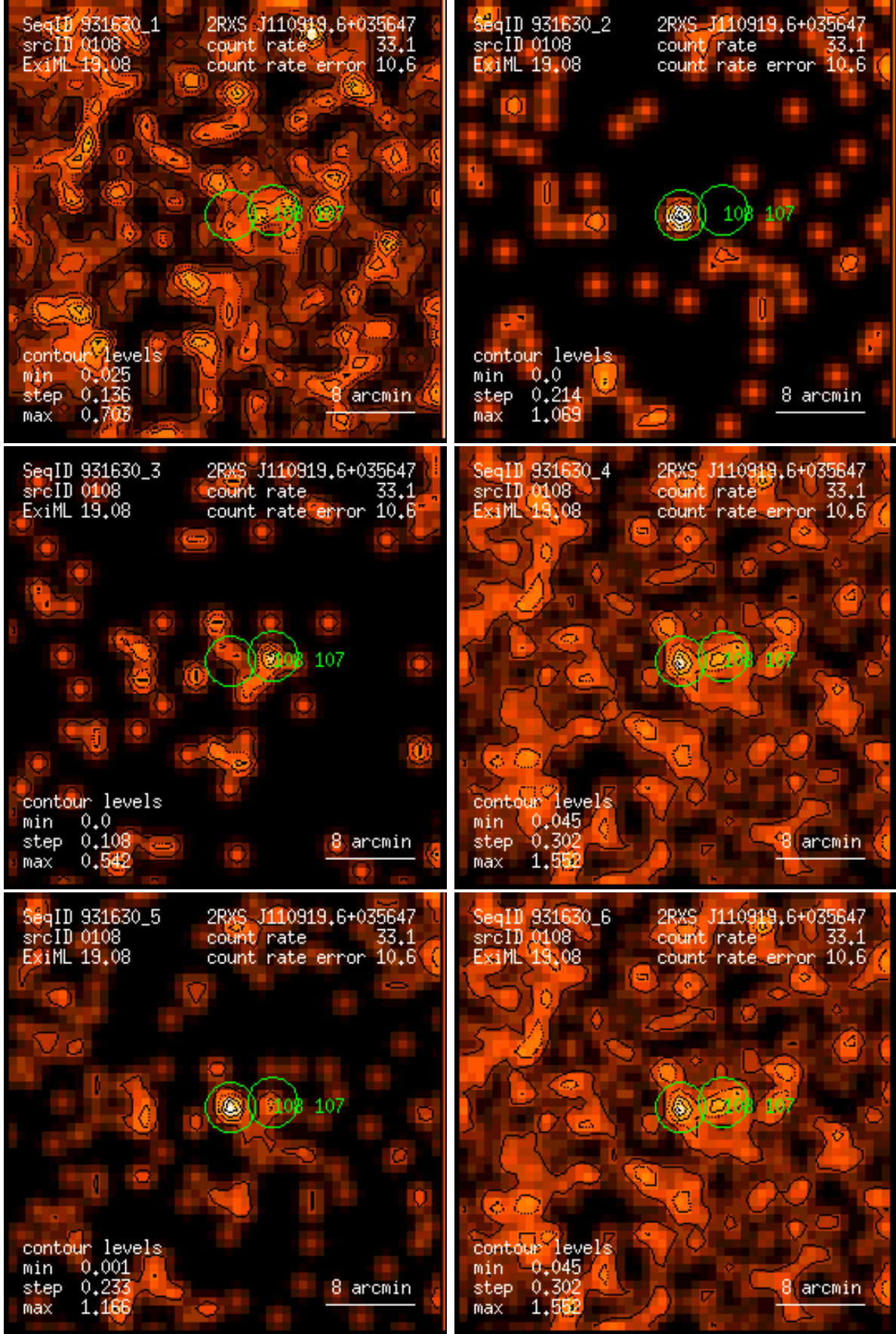
Figure 108: RASS 931630: detection 0108: band rate images, Gaussian filter: (1) PSPC channels 11 – 41, (2) 52 – 90, (3) 91 – 201, (4) 11 – 235, (5) 52 – 201, (6) 11 – 201. Broad band rates in counts/ks. Band rate contour levels in counts/ks/arcmin 2 .
