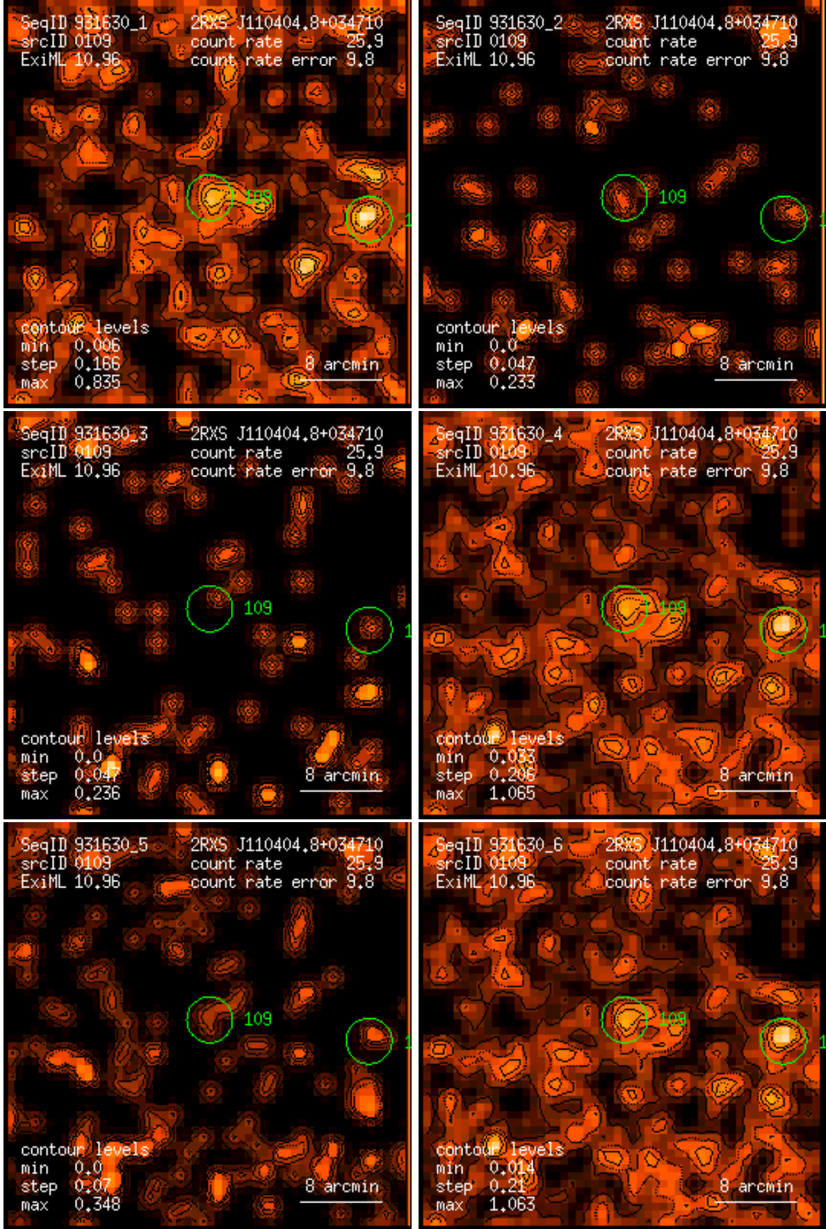
Figure 109: RASS 931630: detection 0109: band rate images, Gaussian filter: (1) PSPC channels 11 – 41, (2) 52 – 90, (3) 91 – 201, (4) 11 – 235, (5) 52 – 201, (6) 11 – 201. Broad band rates in counts/ks. Band rate contour levels in counts/ks/arcmin 2 .
