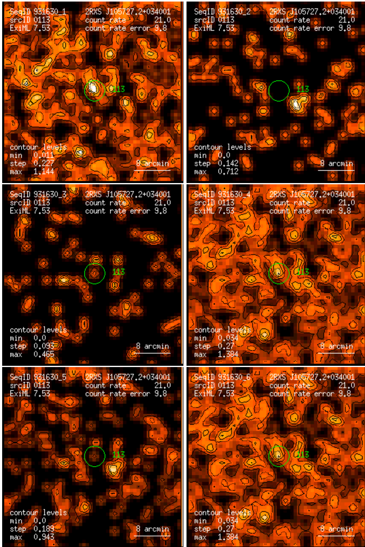
Figure 113: RASS 931630: detection 0113: band rate images, Gaussian filter: (1) PSPC channels 11 – 41, (2) 52 – 90, (3) 91 – 201, (4) 11 – 235, (5) 52 – 201, (6) 11 – 201. Broad band rates in counts/ks. Band rate contour levels in counts/ks/arcmin 2 .
