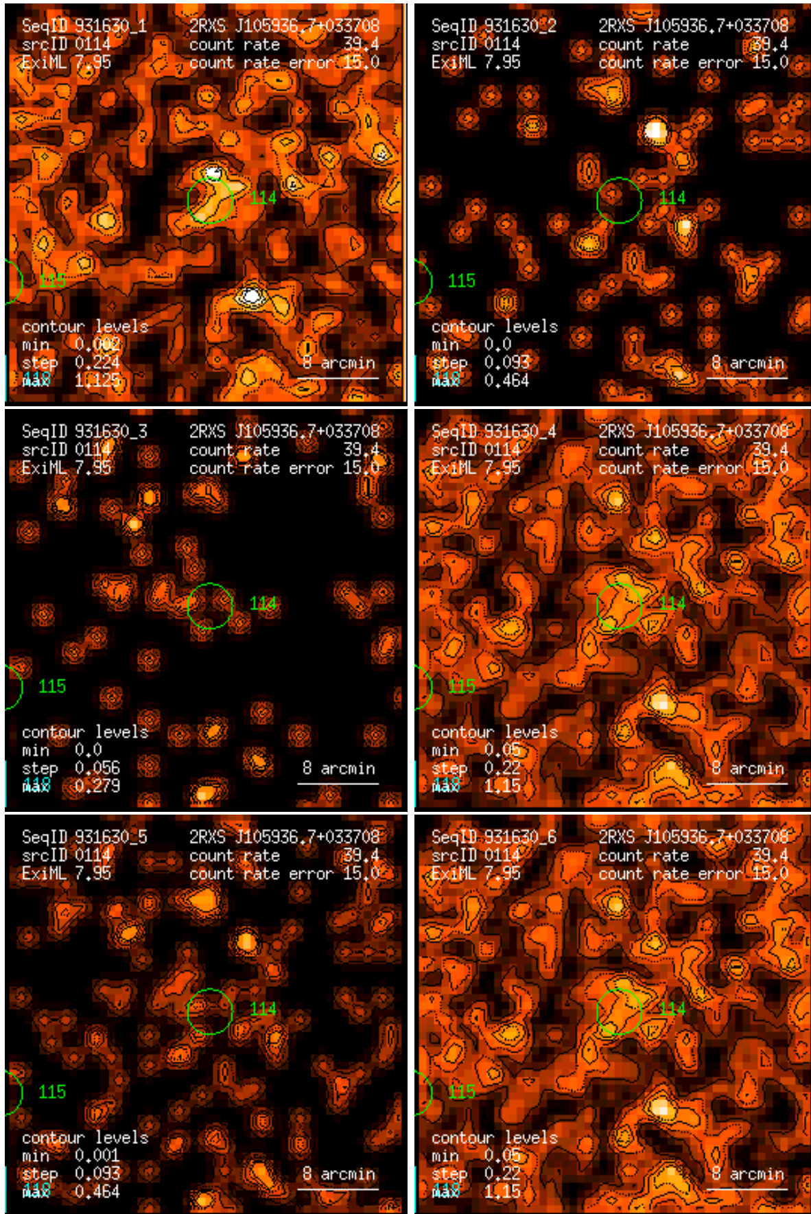
Figure 114: RASS 931630: detection 0114: band rate images, Gaussian filter: (1) PSPC channels 11 – 41, (2) 52 – 90, (3) 91 – 201, (4) 11 – 235, (5) 52 – 201, (6) 11 – 201. Broad band rates in counts/ks. Band rate contour levels in counts/ks/arcmin 2 .
