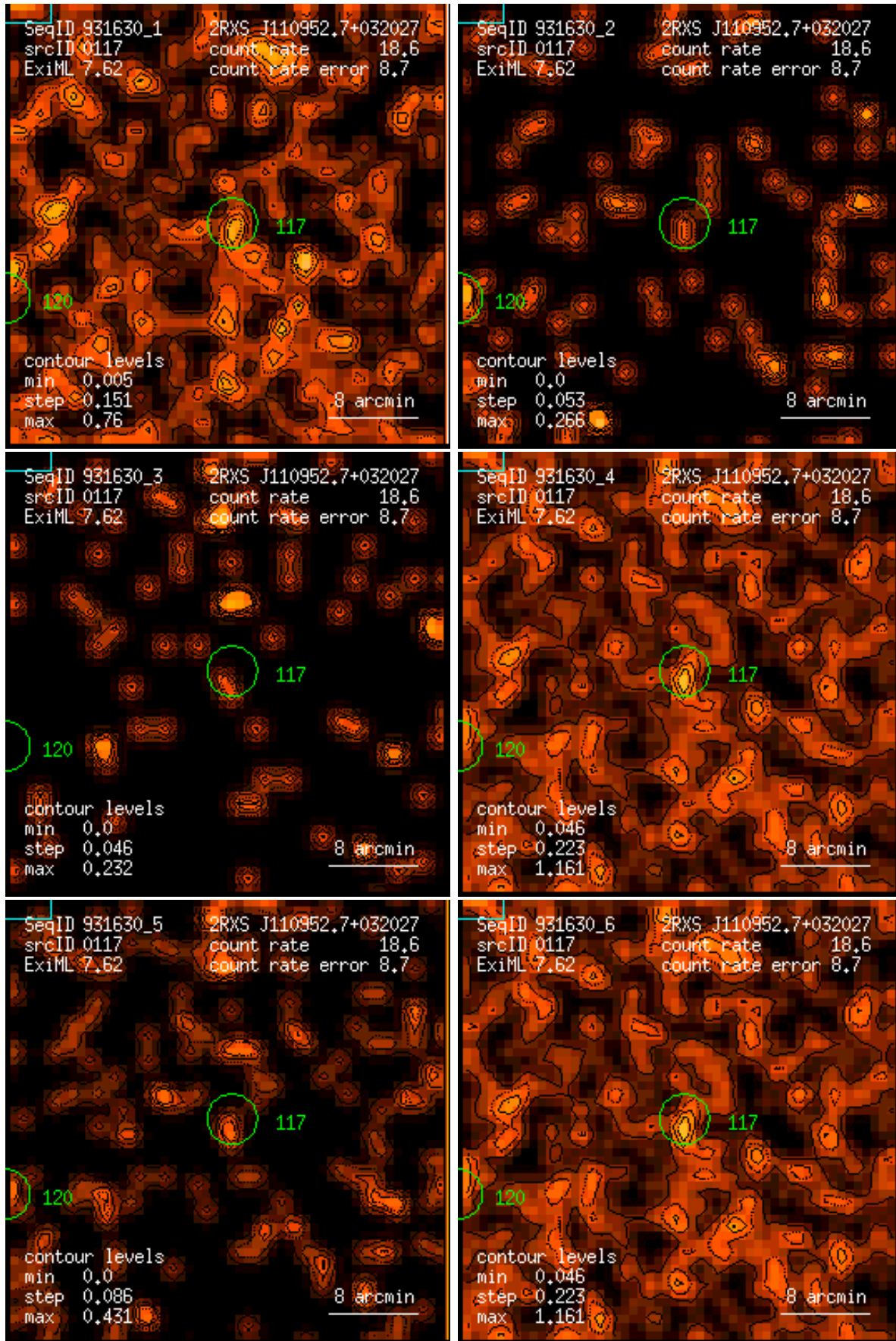
Figure 117: RASS 931630: detection 0117: band rate images, Gaussian filter: (1) PSPC channels 11 – 41, (2) 52 – 90, (3) 91 – 201, (4) 11 – 235, (5) 52 – 201, (6) 11 – 201. Broad band rates in counts/ks. Band rate contour levels in counts/ks/arcmin 2 .
