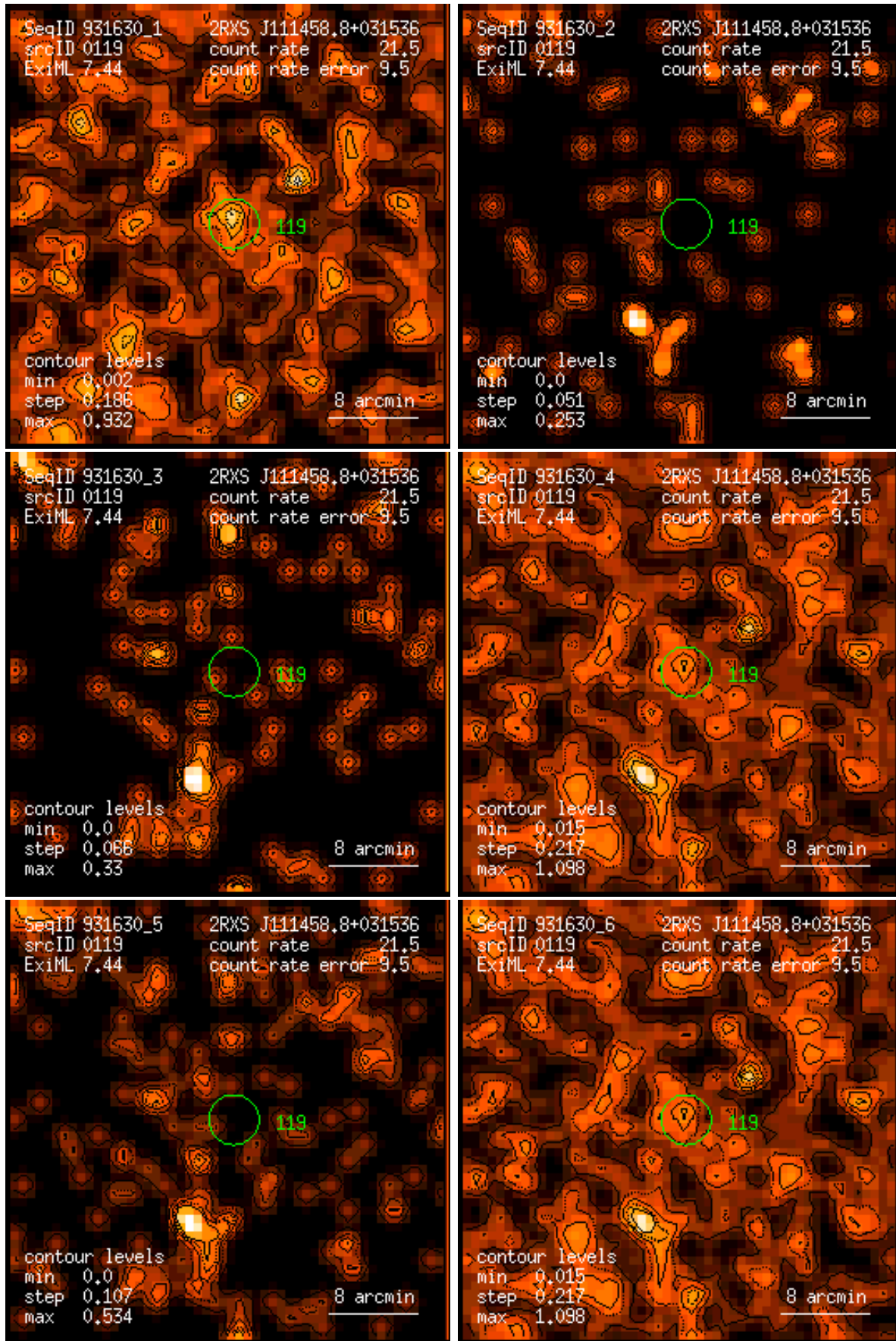
Figure 119: RASS 931630: detection 0119: band rate images, Gaussian filter: (1) PSPC channels 11 – 41, (2) 52 – 90, (3) 91 – 201, (4) 11 – 235, (5) 52 – 201, (6) 11 – 201. Broad band rates in counts/ks. Band rate contour levels in counts/ks/arcmin 2 .
