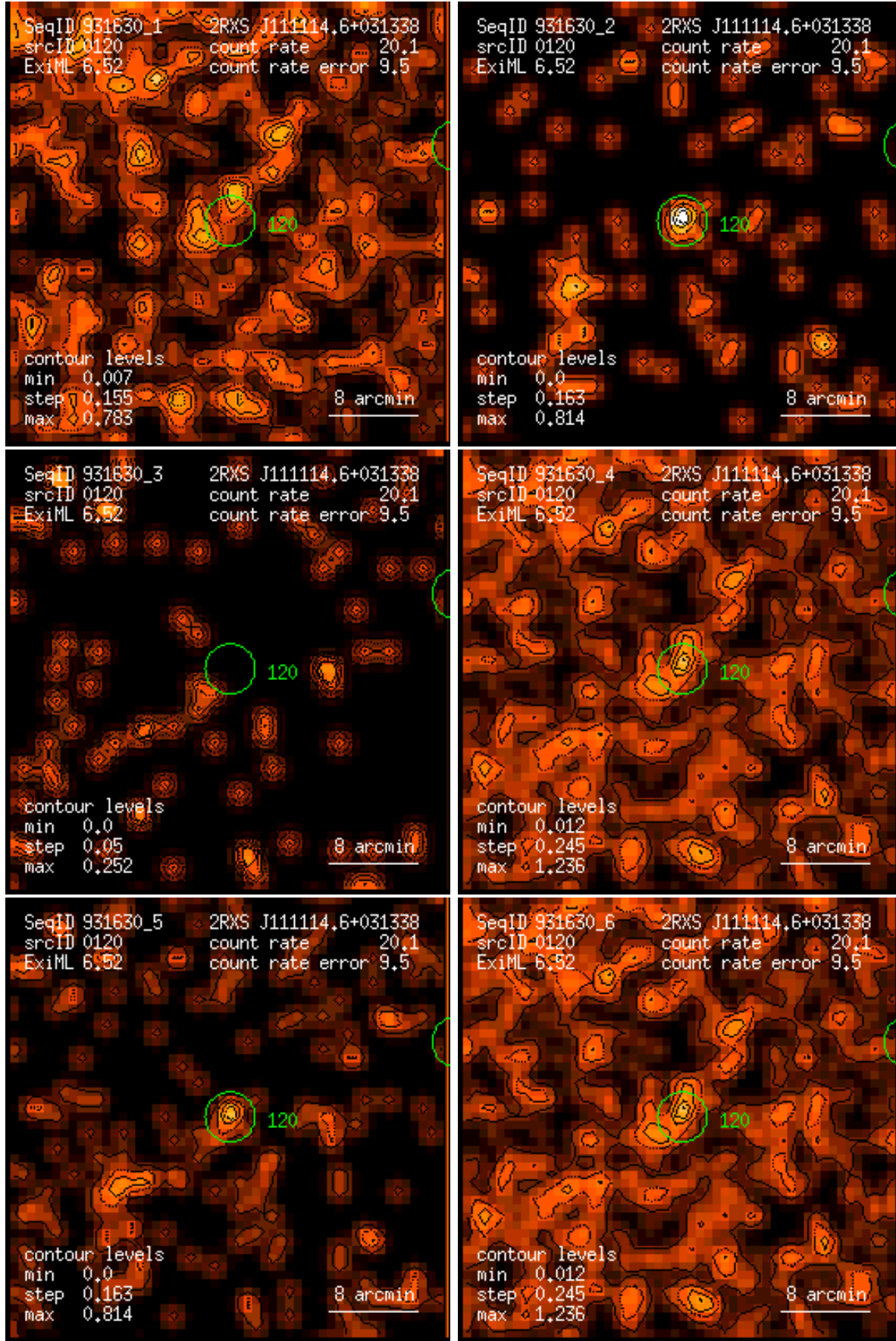
Figure 120: RASS 931630: detection 0120: band rate images, Gaussian filter: (1) PSPC channels 11 – 41, (2) 52 – 90, (3) 91 – 201, (4) 11 – 235, (5) 52 – 201, (6) 11 – 201. Broad band rates in counts/ks. Band rate contour levels in counts/ks/arcmin 2 .
