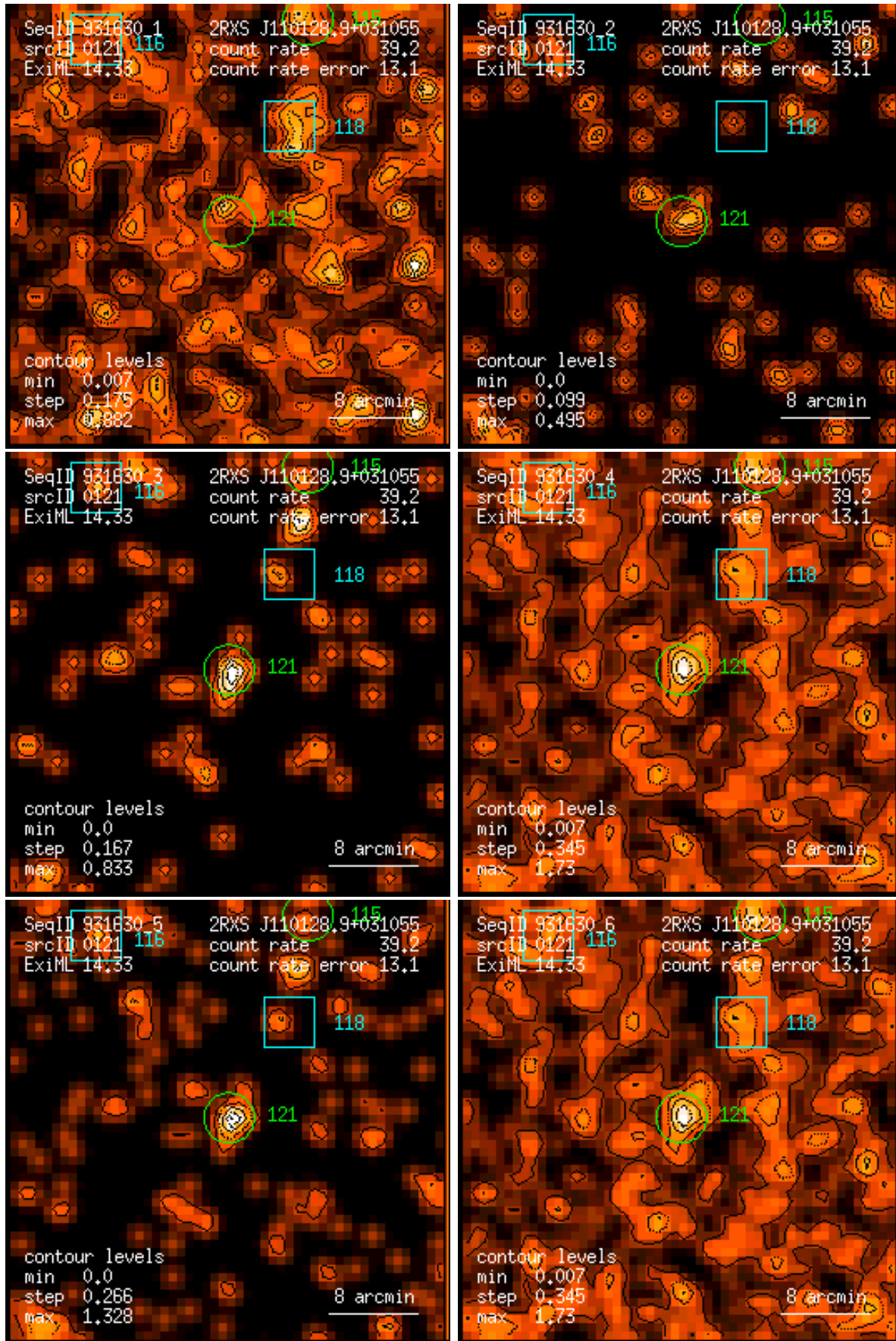
Figure 121: RASS 931630: detection 0121: band rate images, Gaussian filter: (1) PSPC channels 11 – 41, (2) 52 – 90, (3) 91 – 201, (4) 11 – 235, (5) 52 – 201, (6) 11 – 201. Broad band rates in counts/ks. Band rate contour levels in counts/ks/arcmin 2 .
