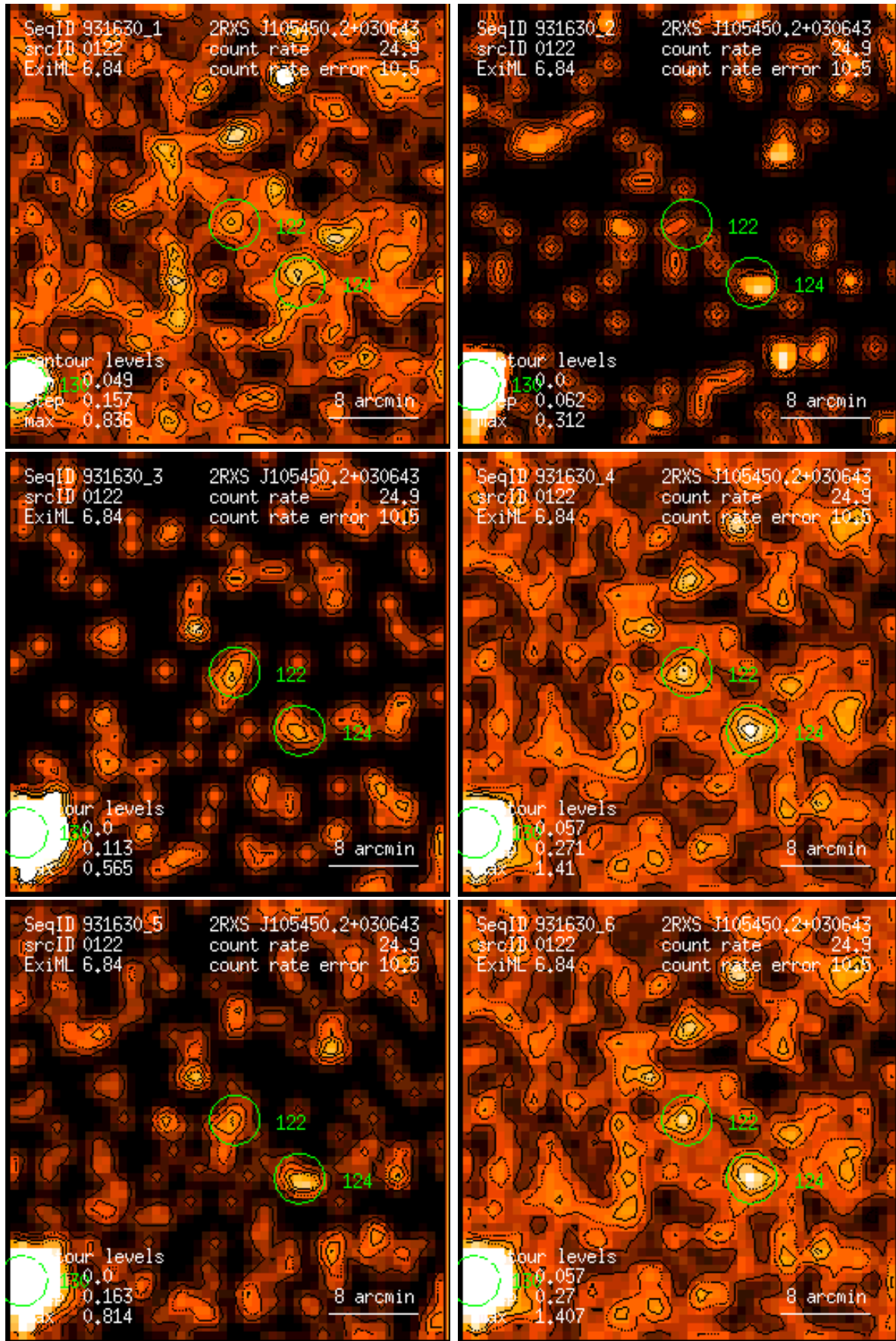
Figure 122: RASS 931630: detection 0122: band rate images, Gaussian filter: (1) PSPC channels 11 – 41, (2) 52 – 90, (3) 91 – 201, (4) 11 – 235, (5) 52 – 201, (6) 11 – 201. Broad band rates in counts/ks. Band rate contour levels in counts/ks/arcmin 2 .
