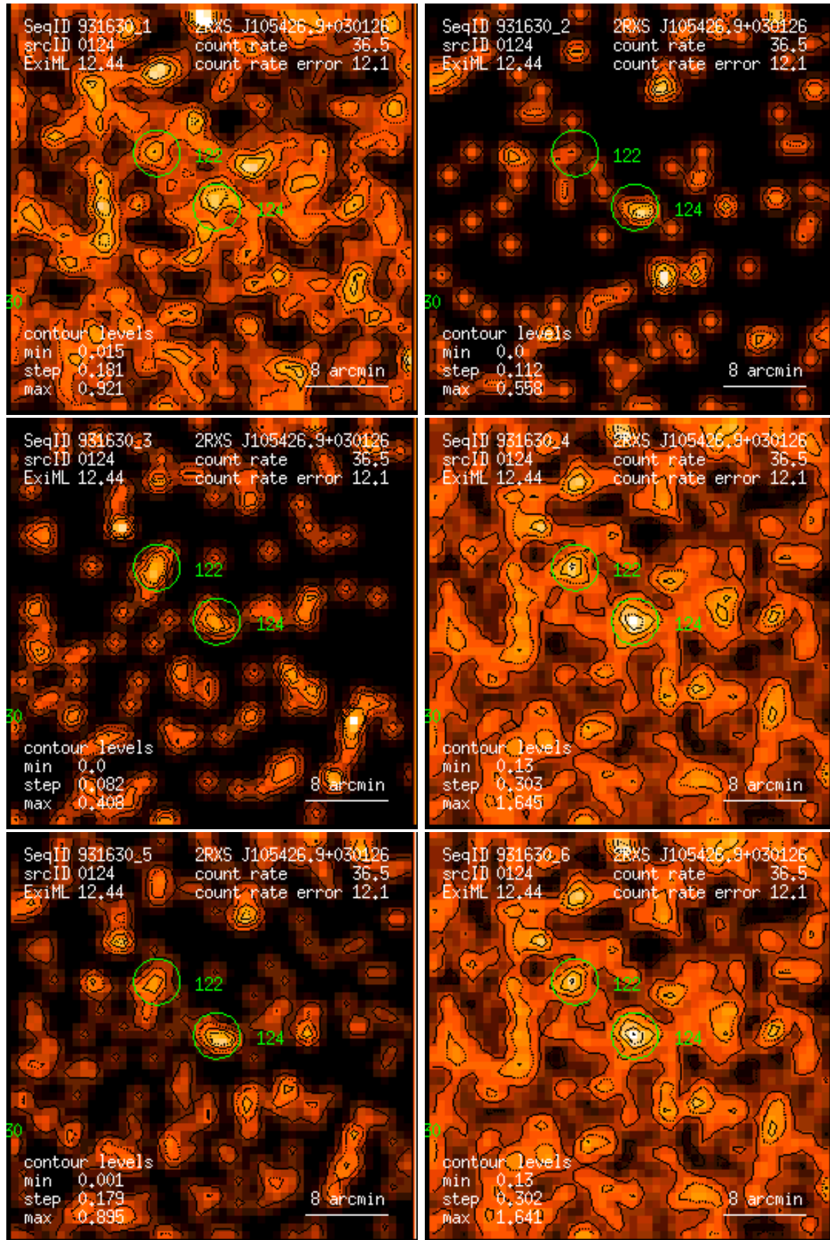
Figure 124: RASS 931630: detection 0124: band rate images, Gaussian filter: (1) PSPC channels 11 – 41, (2) 52 – 90, (3) 91 – 201, (4) 11 – 235, (5) 52 – 201, (6) 11 – 201. Broad band rates in counts/ks. Band rate contour levels in counts/ks/arcmin 2 .
