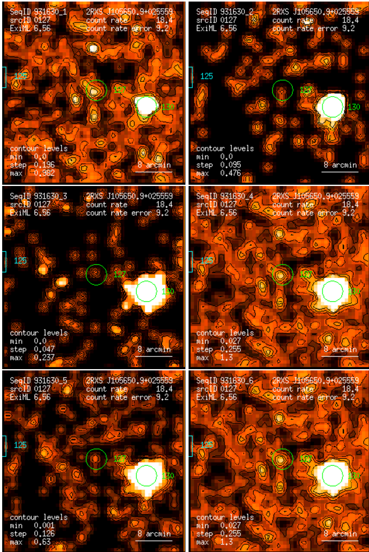
Figure 127: RASS 931630: detection 0127: band rate images, Gaussian filter: (1) PSPC channels 11 – 41, (2) 52 – 90, (3) 91 – 201, (4) 11 – 235, (5) 52 – 201, (6) 11 – 201. Broad band rates in counts/ks. Band rate contour levels in counts/ks/arcmin 2 .
