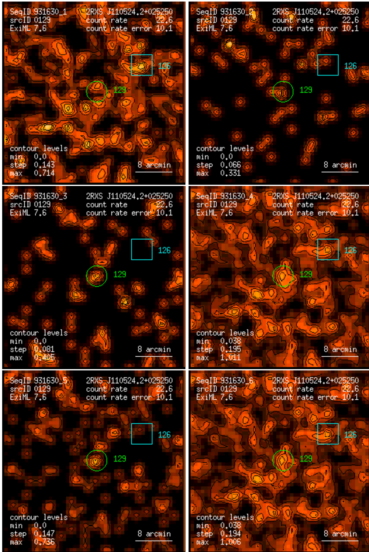
Figure 129: RASS 931630: detection 0129: band rate images, Gaussian filter: (1) PSPC channels 11 – 41, (2) 52 – 90, (3) 91 – 201, (4) 11 – 235, (5) 52 – 201, (6) 11 – 201. Broad band rates in counts/ks. Band rate contour levels in counts/ks/arcmin 2 .
