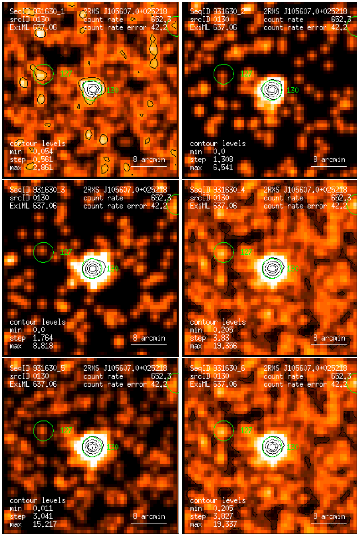
Figure 130: RASS 931630: detection 0130: band rate images, Gaussian filter: (1) PSPC channels 11 – 41, (2) 52 – 90, (3) 91 – 201, (4) 11 – 235, (5) 52 – 201, (6) 11 – 201. Broad band rates in counts/ks. Band rate contour levels in counts/ks/arcmin 2 .
