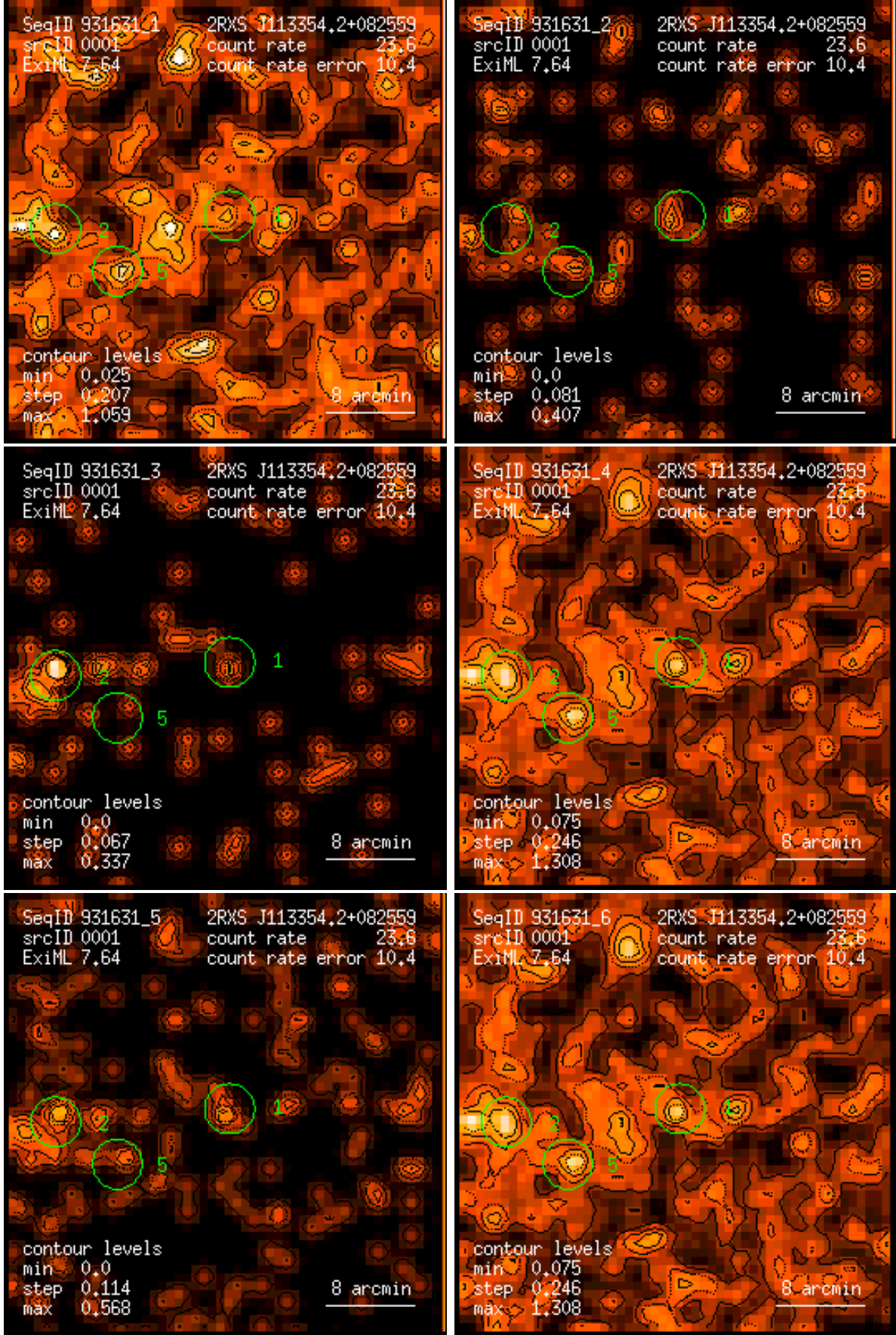
Figure 1: RASS 931631: detection 0001: band rate images, Gaussian filter: (1) PSPC channels 11 – 41, (2) 52 – 90, (3) 91 – 201, (4) 11 – 235, (5) 52 – 201, (6) 11 – 201. Broad band rates in counts/ks. Band rate contour levels in counts/ks/arcmin 2 .
