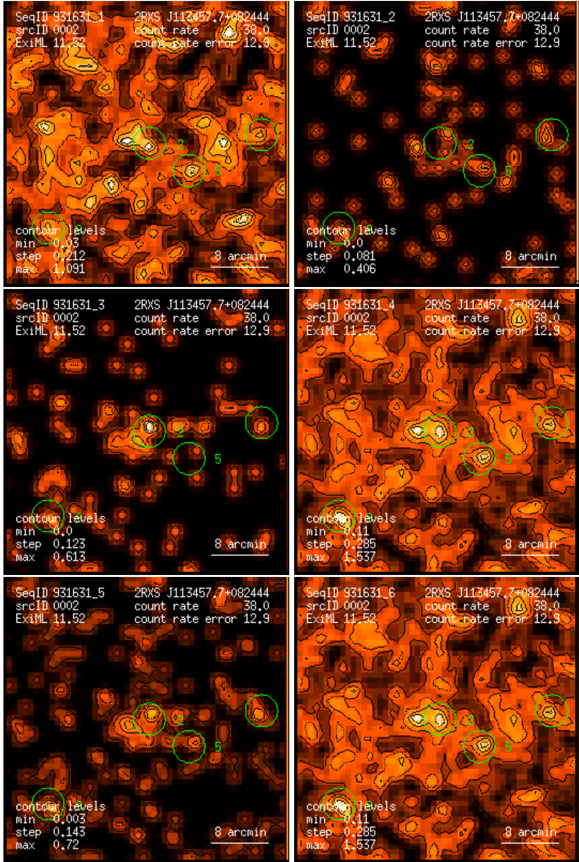
Figure 2: RASS 931631: detection 0002: band rate images, Gaussian filter: (1) PSPC channels 11 – 41, (2) 52 – 90, (3) 91 – 201, (4) 11 – 235, (5) 52 – 201, (6) 11 – 201. Broad band rates in counts/ks. Band rate contour levels in counts/ks/arcmin 2 .
