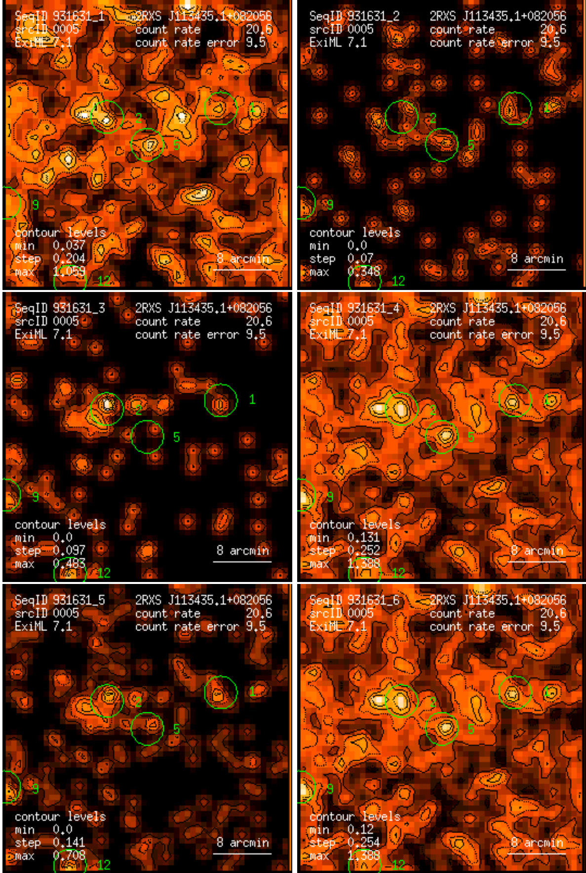
Figure 5: RASS 931631: detection 0005: band rate images, Gaussian filter: (1) PSPC channels 11 – 41, (2) 52 – 90, (3) 91 – 201, (4) 11 – 235, (5) 52 – 201, (6) 11 – 201. Broad band rates in counts/ks. Band rate contour levels in counts/ks/arcmin 2 .
