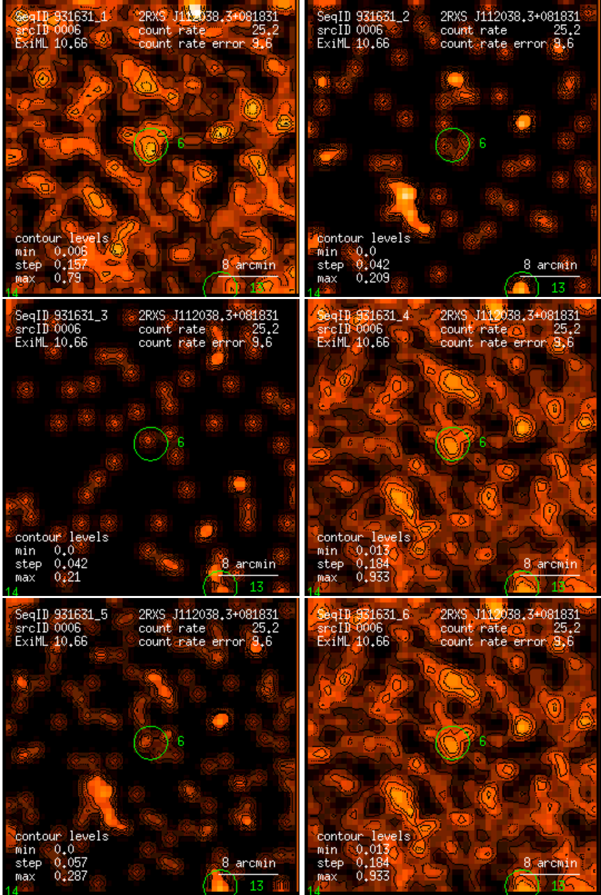
Figure 6: RASS 931631: detection 0006: band rate images, Gaussian filter: (1) PSPC channels 11 – 41, (2) 52 – 90, (3) 91 – 201, (4) 11 – 235, (5) 52 – 201, (6) 11 – 201. Broad band rates in counts/ks. Band rate contour levels in counts/ks/arcmin 2 .
