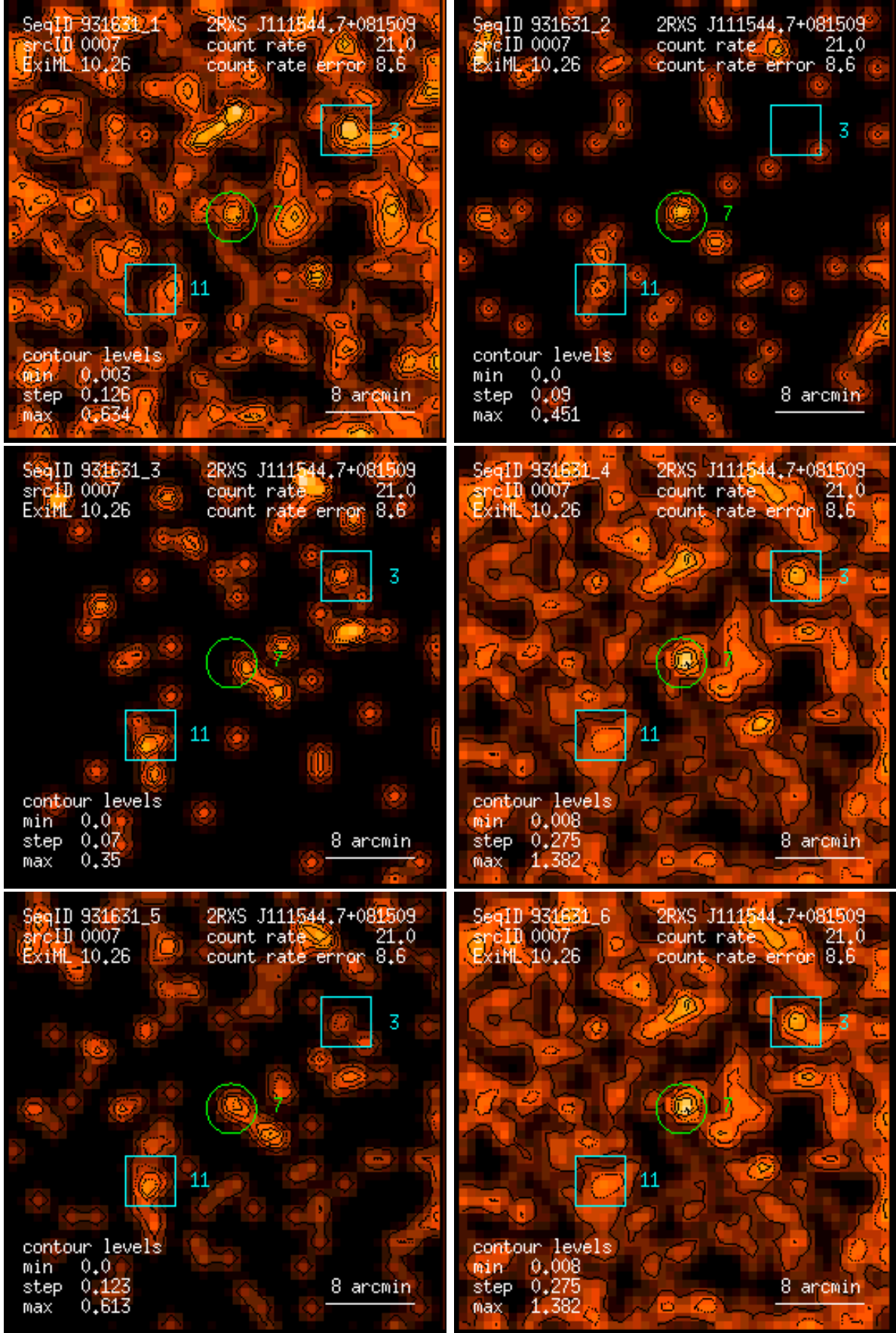
Figure 7: RASS 931631: detection 0007: band rate images, Gaussian filter: (1) PSPC channels 11 – 41, (2) 52 – 90, (3) 91 – 201, (4) 11 – 235, (5) 52 – 201, (6) 11 – 201. Broad band rates in counts/ks. Band rate contour levels in counts/ks/arcmin 2 .
