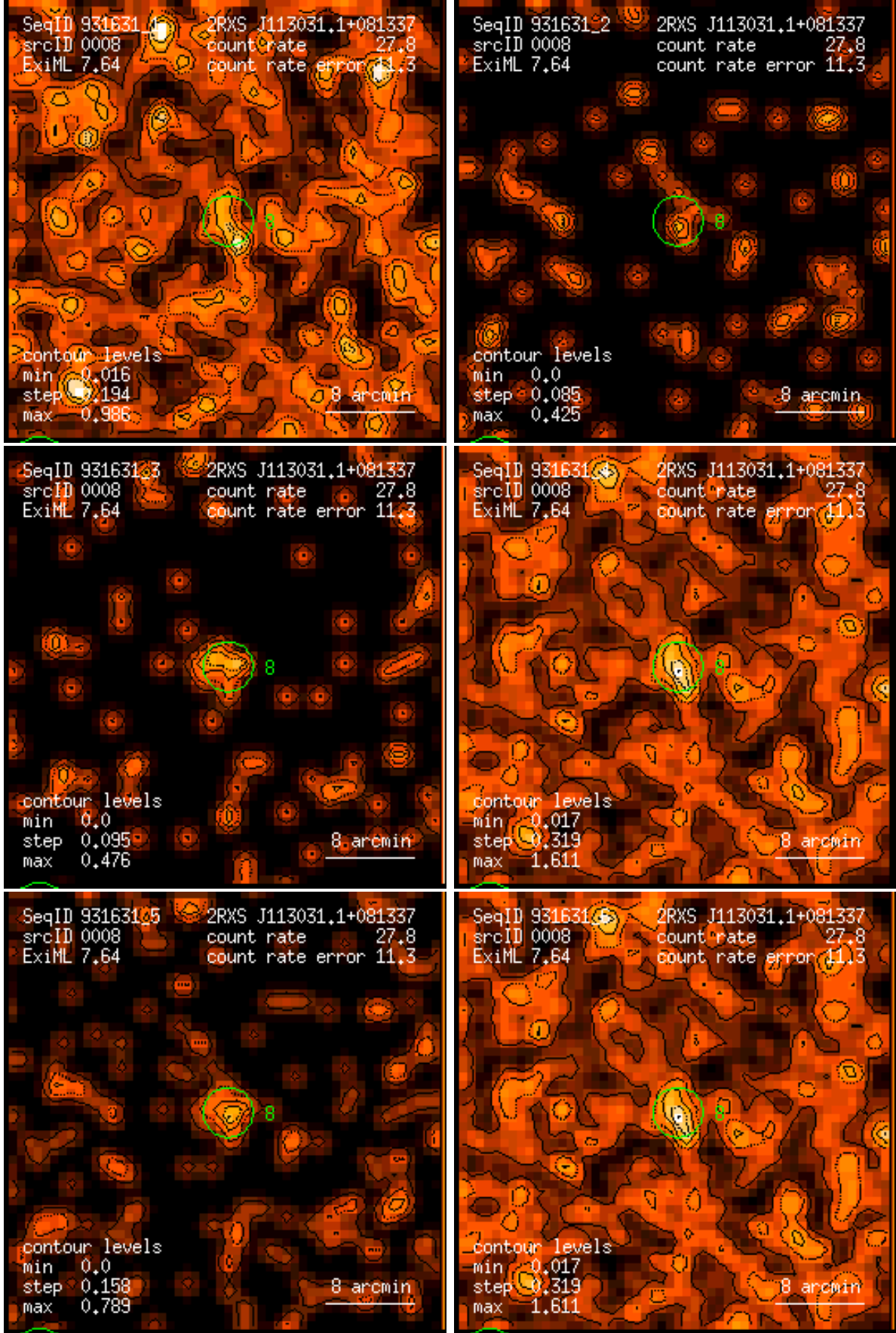
Figure 8: RASS 931631: detection 0008: band rate images, Gaussian filter: (1) PSPC channels 11 – 41, (2) 52 – 90, (3) 91 – 201, (4) 11 – 235, (5) 52 – 201, (6) 11 – 201. Broad band rates in counts/ks. Band rate contour levels in counts/ks/arcmin 2 .
