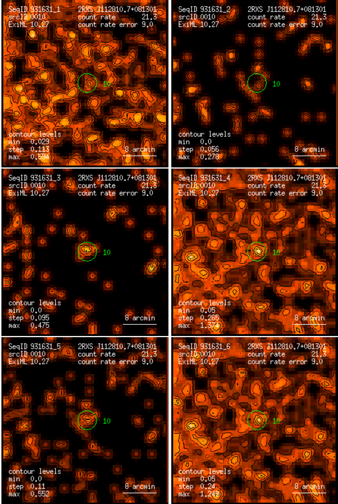
Figure 10: RASS 931631: detection 0010: band rate images, Gaussian filter: (1) PSPC channels 11 – 41, (2) 52 – 90, (3) 91 – 201, (4) 11 – 235, (5) 52 – 201, (6) 11 – 201. Broad band rates in counts/ks. Band rate contour levels in counts/ks/arcmin 2 .
