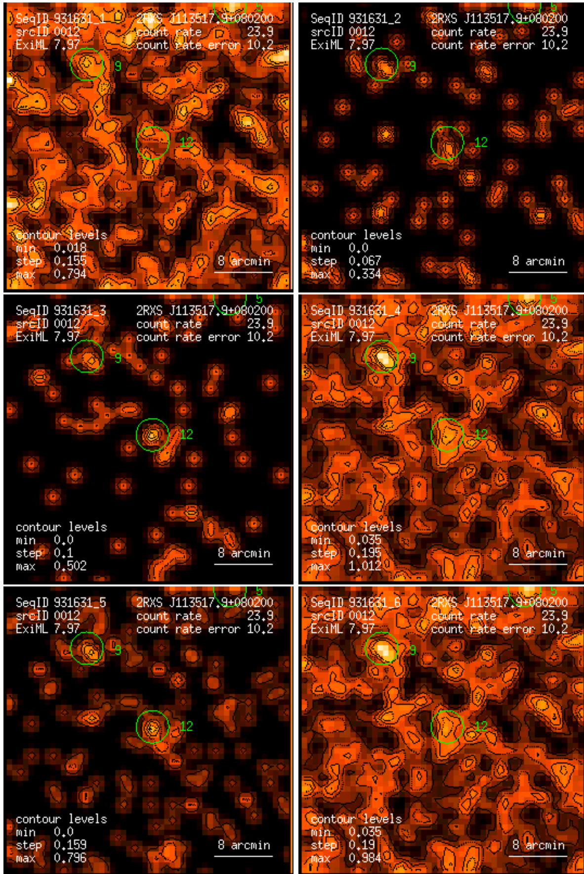
Figure 12: RASS 931631: detection 0012: band rate images, Gaussian filter: (1) PSPC channels 11 – 41, (2) 52 – 90, (3) 91 – 201, (4) 11 – 235, (5) 52 – 201, (6) 11 – 201. Broad band rates in counts/ks. Band rate contour levels in counts/ks/arcmin 2 .
