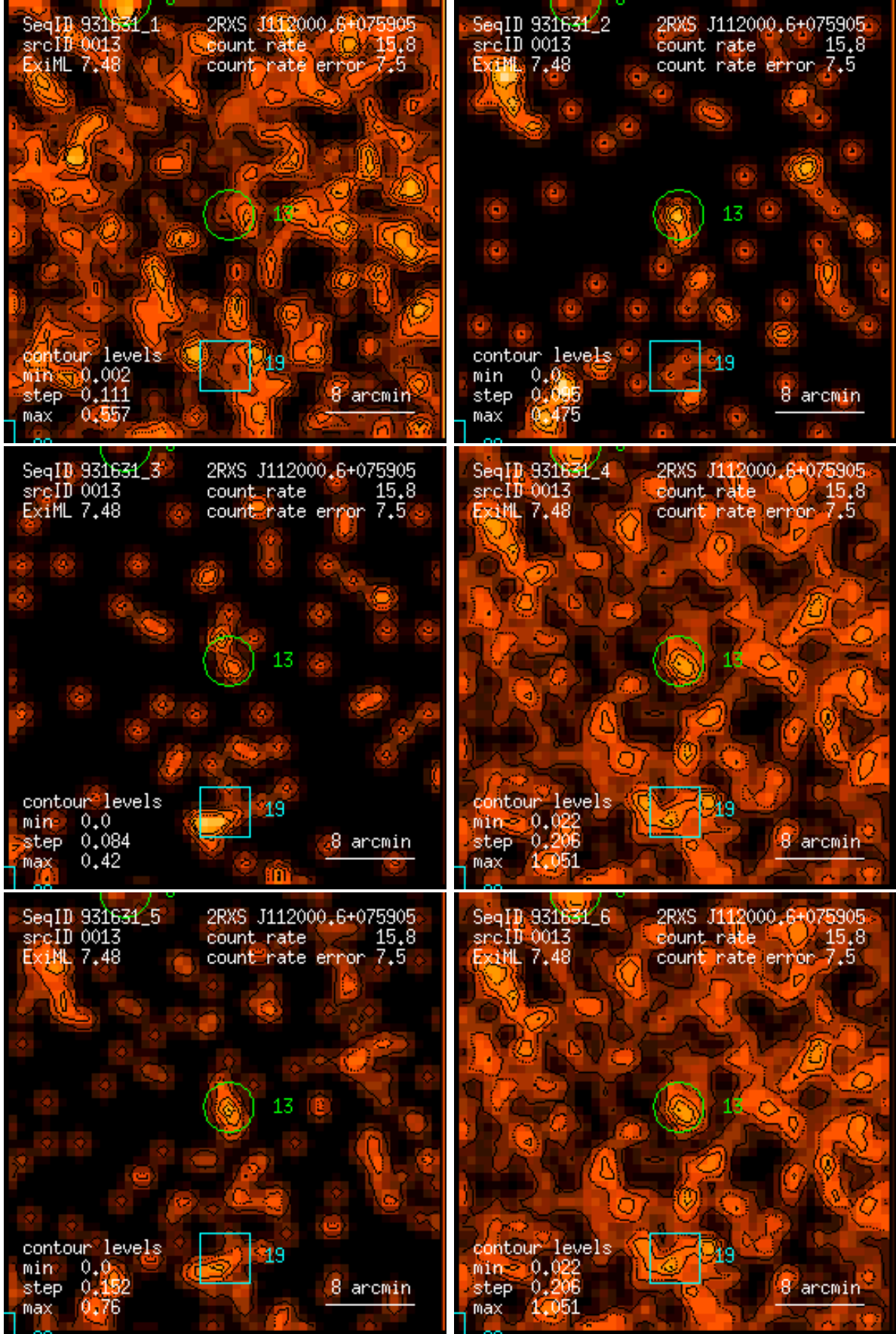
Figure 13: RASS 931631: detection 0013: band rate images, Gaussian filter: (1) PSPC channels 11 – 41, (2) 52 – 90, (3) 91 – 201, (4) 11 – 235, (5) 52 – 201, (6) 11 – 201. Broad band rates in counts/ks. Band rate contour levels in counts/ks/arcmin 2 .
