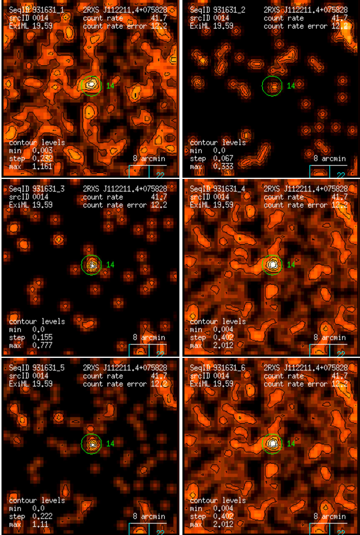
Figure 14: RASS 931631: detection 0014: band rate images, Gaussian filter: (1) PSPC channels 11 – 41, (2) 52 – 90, (3) 91 – 201, (4) 11 – 235, (5) 52 – 201, (6) 11 – 201. Broad band rates in counts/ks. Band rate contour levels in counts/ks/arcmin 2 .
