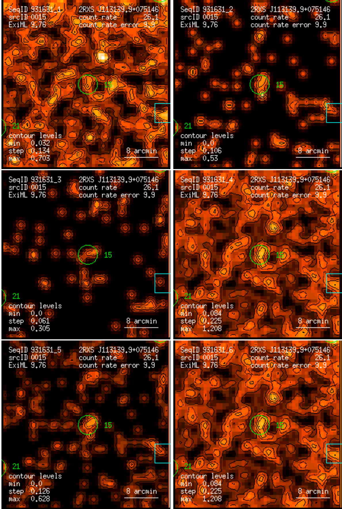
Figure 15: RASS 931631: detection 0015: band rate images, Gaussian filter: (1) PSPC channels 11 – 41, (2) 52 – 90, (3) 91 – 201, (4) 11 – 235, (5) 52 – 201, (6) 11 – 201. Broad band rates in counts/ks. Band rate contour levels in counts/ks/arcmin 2 .
