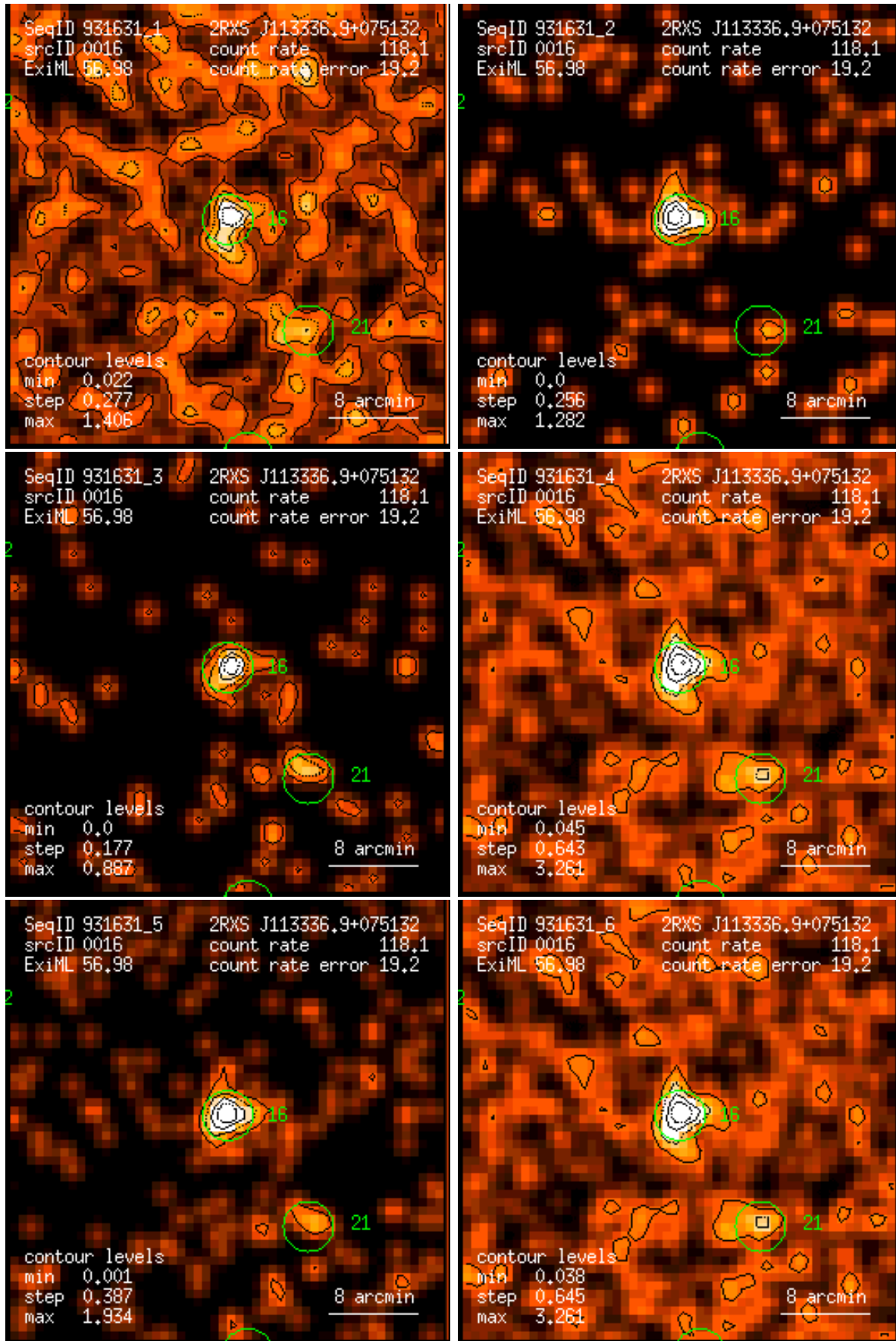
Figure 16: RASS 931631: detection 0016: band rate images, Gaussian filter: (1) PSPC channels 11 – 41, (2) 52 – 90, (3) 91 – 201, (4) 11 – 235, (5) 52 – 201, (6) 11 – 201. Broad band rates in counts/ks. Band rate contour levels in counts/ks/arcmin 2 .
