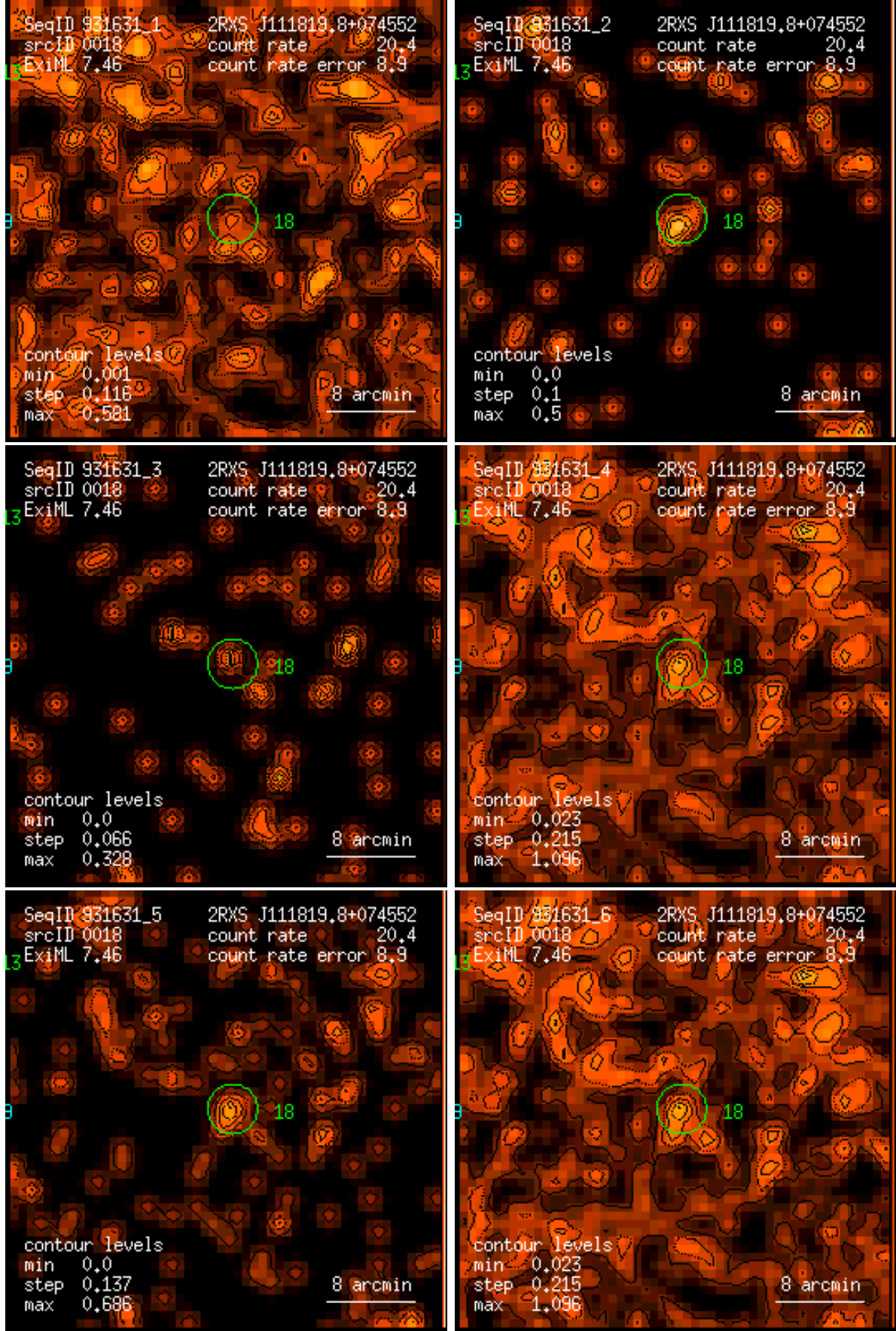
Figure 18: RASS 931631: detection 0018: band rate images, Gaussian filter: (1) PSPC channels 11 – 41, (2) 52 – 90, (3) 91 – 201, (4) 11 – 235, (5) 52 – 201, (6) 11 – 201. Broad band rates in counts/ks. Band rate contour levels in counts/ks/arcmin 2 .
