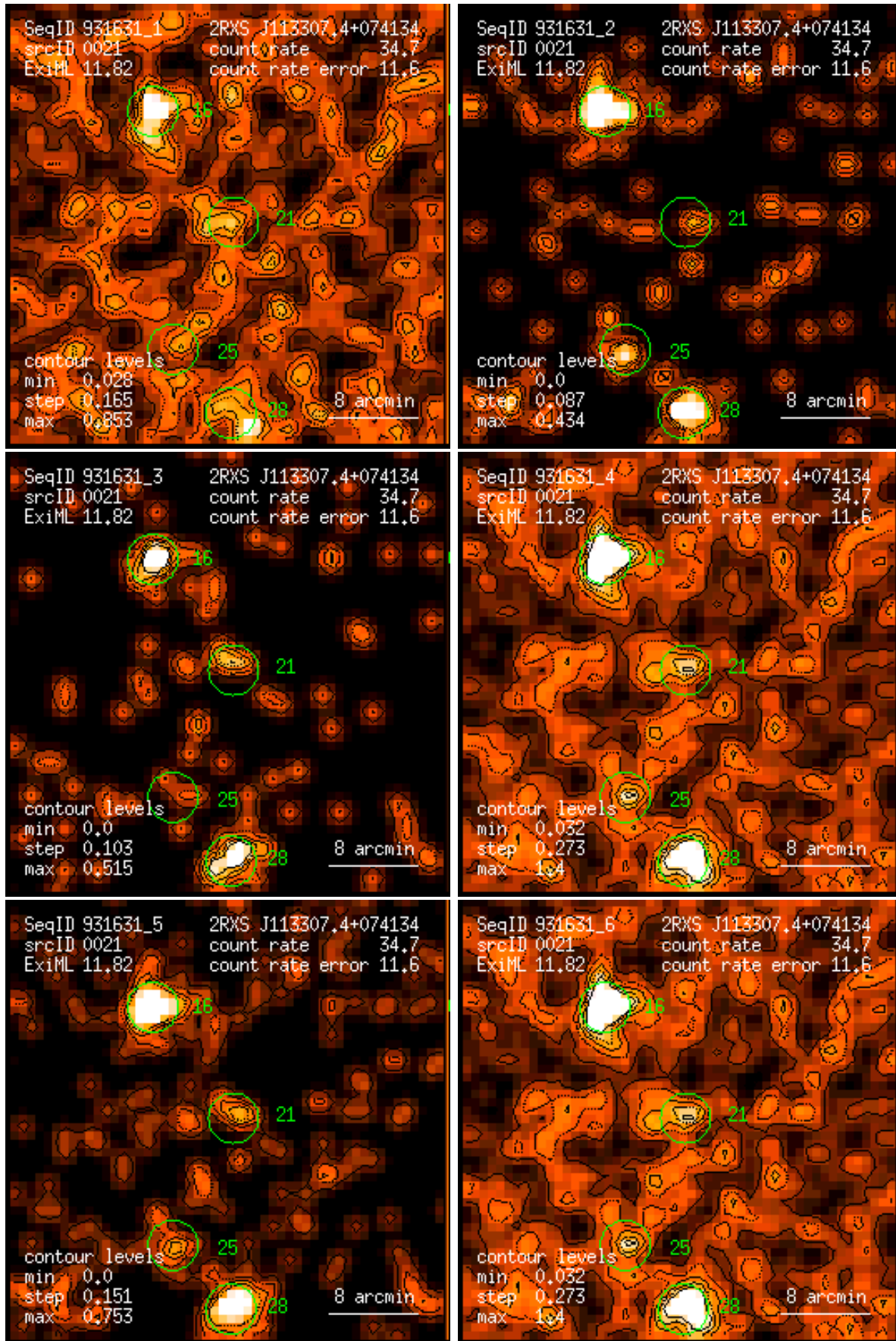
Figure 21: RASS 931631: detection 0021: band rate images, Gaussian filter: (1) PSPC channels 11 – 41, (2) 52 – 90, (3) 91 – 201, (4) 11 – 235, (5) 52 – 201, (6) 11 – 201. Broad band rates in counts/ks. Band rate contour levels in counts/ks/arcmin 2 .
