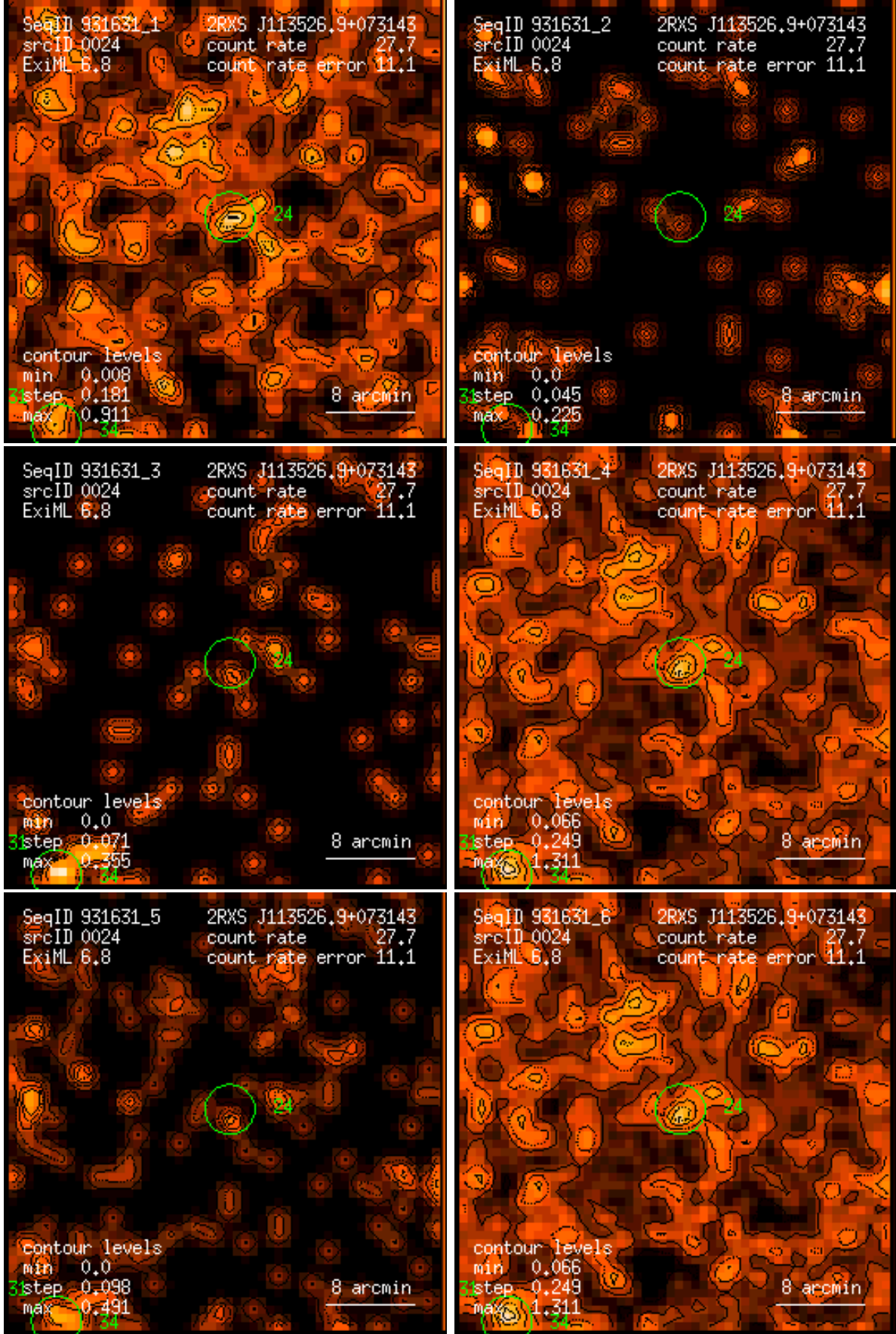
Figure 24: RASS 931631: detection 0024: band rate images, Gaussian filter: (1) PSPC channels 11 – 41, (2) 52 – 90, (3) 91 – 201, (4) 11 – 235, (5) 52 – 201, (6) 11 – 201. Broad band rates in counts/ks. Band rate contour levels in counts/ks/arcmin 2 .
