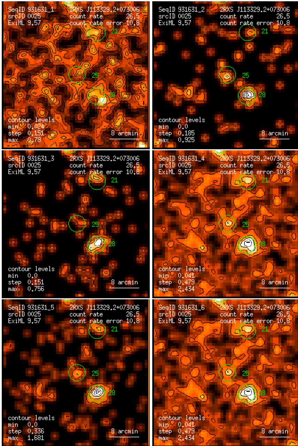
Figure 25: RASS 931631: detection 0025: band rate images, Gaussian filter: (1) PSPC channels 11 – 41, (2) 52 – 90, (3) 91 – 201, (4) 11 – 235, (5) 52 – 201, (6) 11 – 201. Broad band rates in counts/ks. Band rate contour levels in counts/ks/arcmin 2 .
