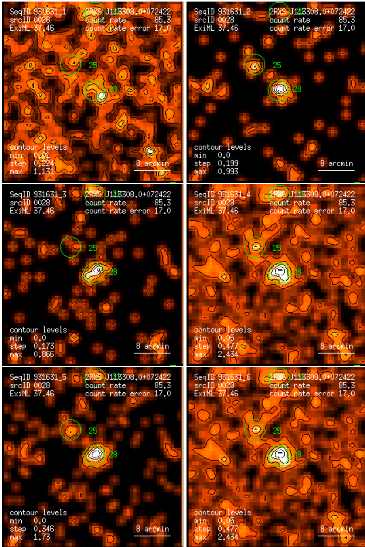
Figure 28: RASS 931631: detection 0028: band rate images, Gaussian filter: (1) PSPC channels 11 – 41, (2) 52 – 90, (3) 91 – 201, (4) 11 – 235, (5) 52 – 201, (6) 11 – 201. Broad band rates in counts/ks. Band rate contour levels in counts/ks/arcmin 2 .
