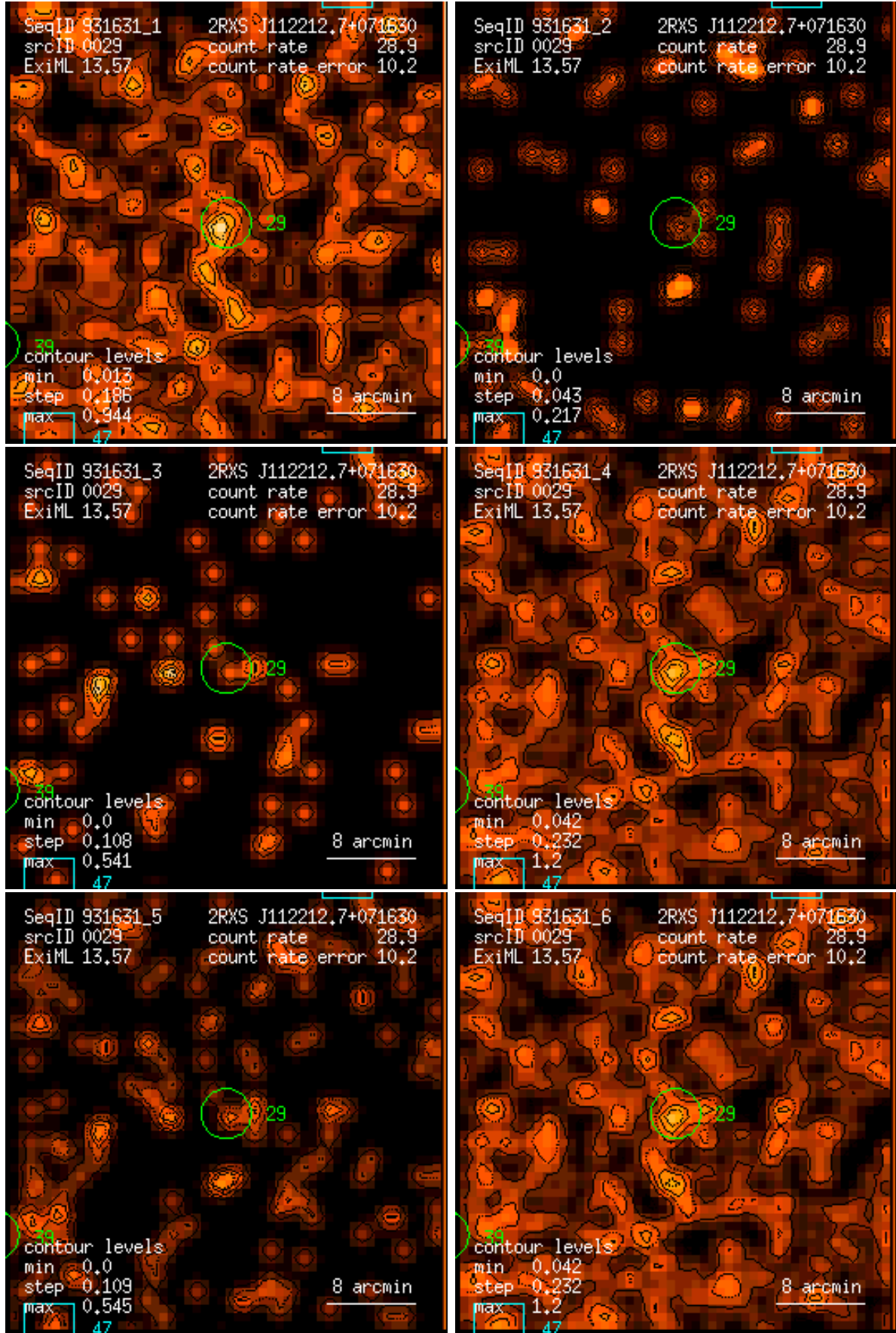
Figure 29: RASS 931631: detection 0029: band rate images, Gaussian filter: (1) PSPC channels 11 – 41, (2) 52 – 90, (3) 91 – 201, (4) 11 – 235, (5) 52 – 201, (6) 11 – 201. Broad band rates in counts/ks. Band rate contour levels in counts/ks/arcmin 2 .
