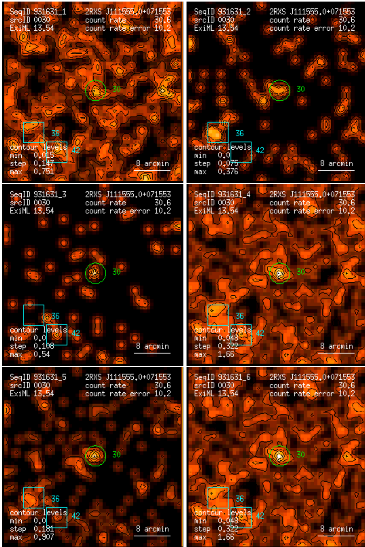
Figure 30: RASS 931631: detection 0030: band rate images, Gaussian filter: (1) PSPC channels 11 – 41, (2) 52 – 90, (3) 91 – 201, (4) 11 – 235, (5) 52 – 201, (6) 11 – 201. Broad band rates in counts/ks. Band rate contour levels in counts/ks/arcmin 2 .
