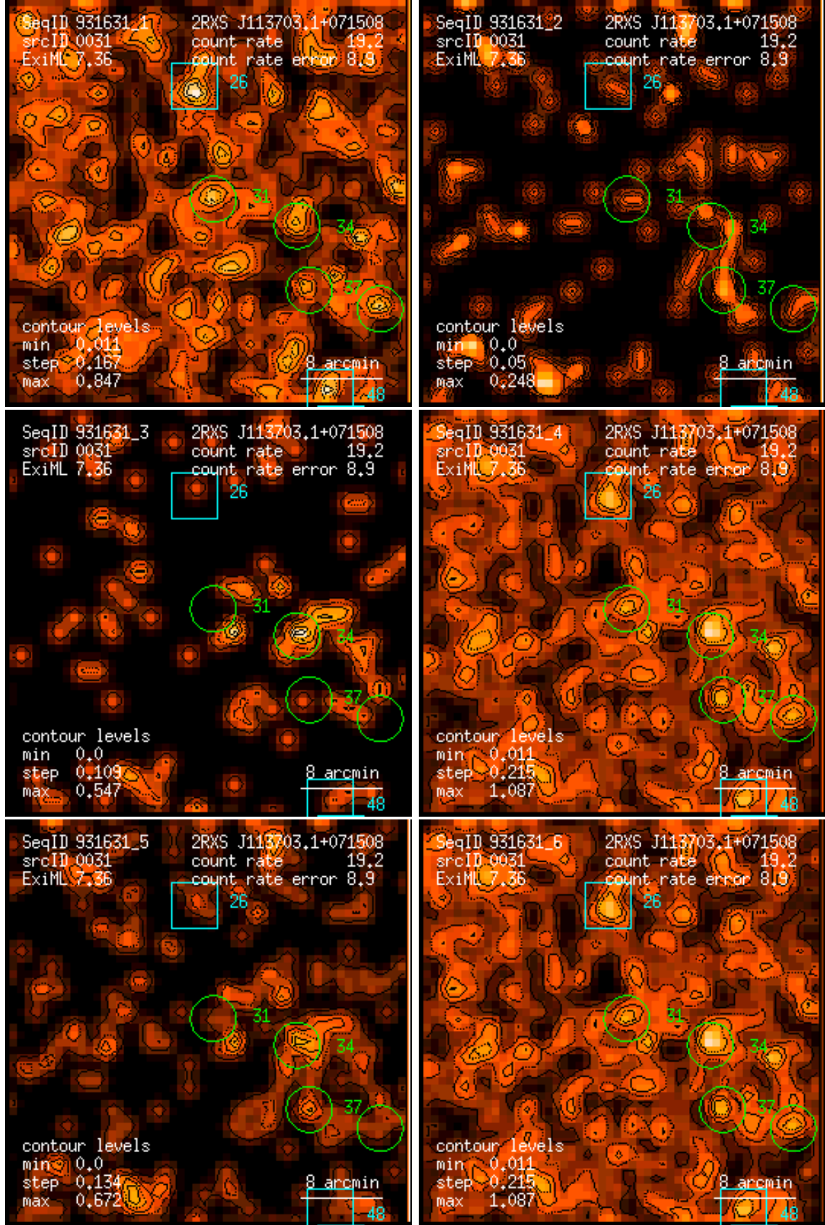
Figure 31: RASS 931631: detection 0031: band rate images, Gaussian filter: (1) PSPC channels 11 – 41, (2) 52 – 90, (3) 91 – 201, (4) 11 – 235, (5) 52 – 201, (6) 11 – 201. Broad band rates in counts/ks. Band rate contour levels in counts/ks/arcmin 2 .
