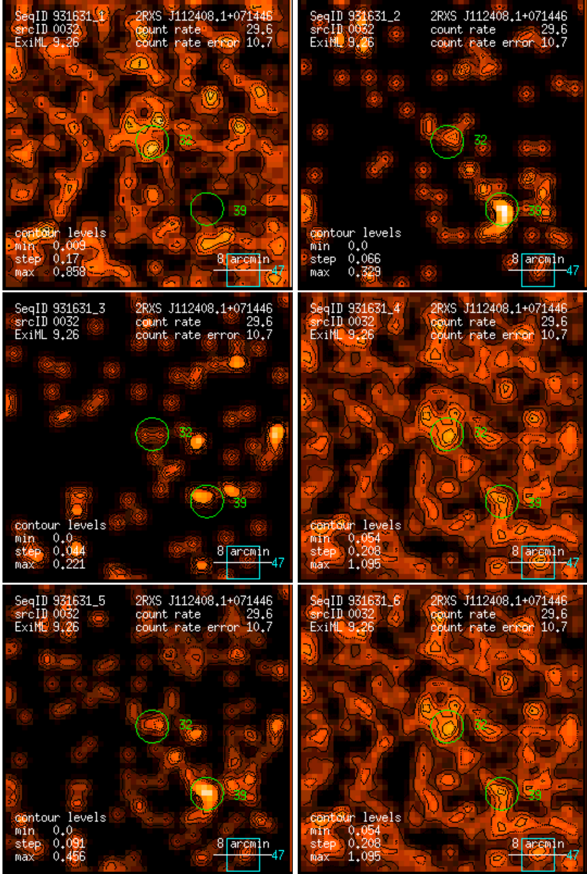
Figure 32: RASS 931631: detection 0032: band rate images, Gaussian filter: (1) PSPC channels 11 – 41, (2) 52 – 90, (3) 91 – 201, (4) 11 – 235, (5) 52 – 201, (6) 11 – 201. Broad band rates in counts/ks. Band rate contour levels in counts/ks/arcmin 2 .
