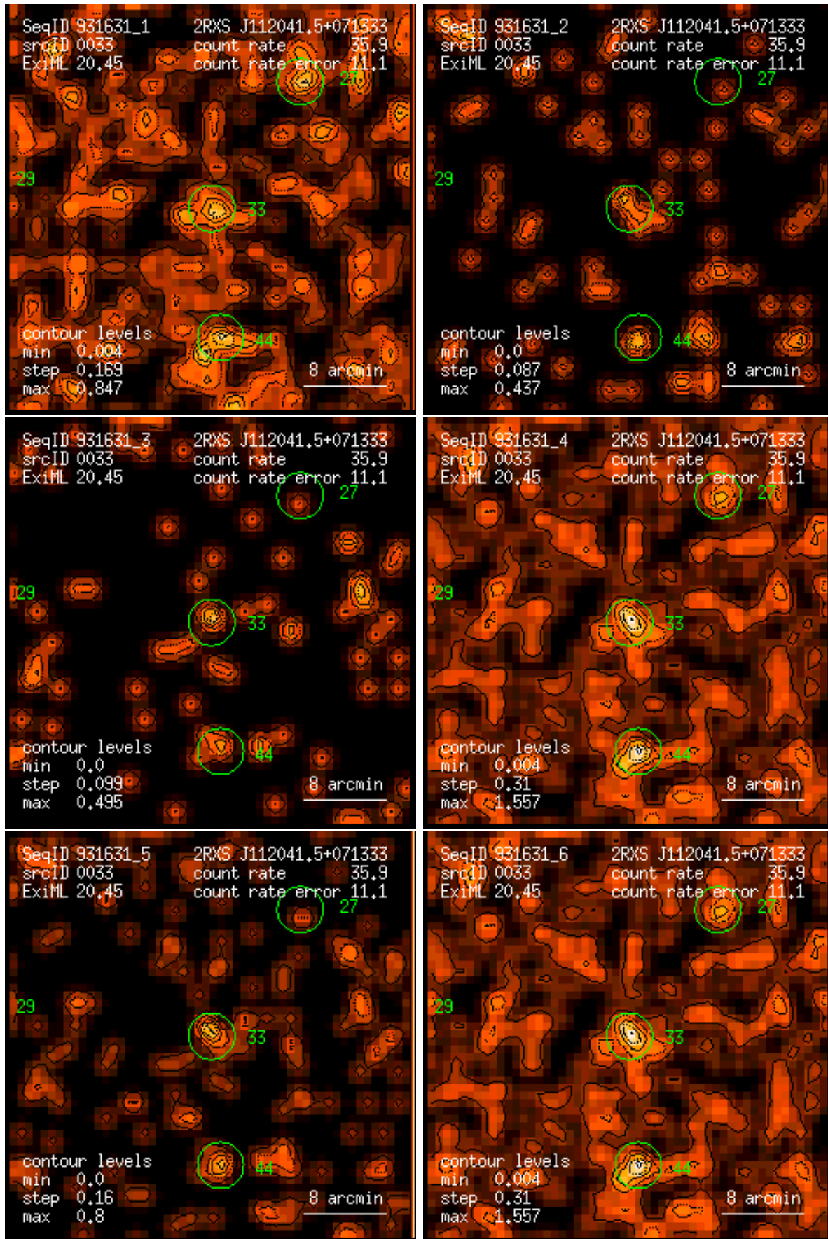
Figure 33: RASS 931631: detection 0033: band rate images, Gaussian filter: (1) PSPC channels 11 – 41, (2) 52 – 90, (3) 91 – 201, (4) 11 – 235, (5) 52 – 201, (6) 11 – 201. Broad band rates in counts/ks. Band rate contour levels in counts/ks/arcmin 2 .
