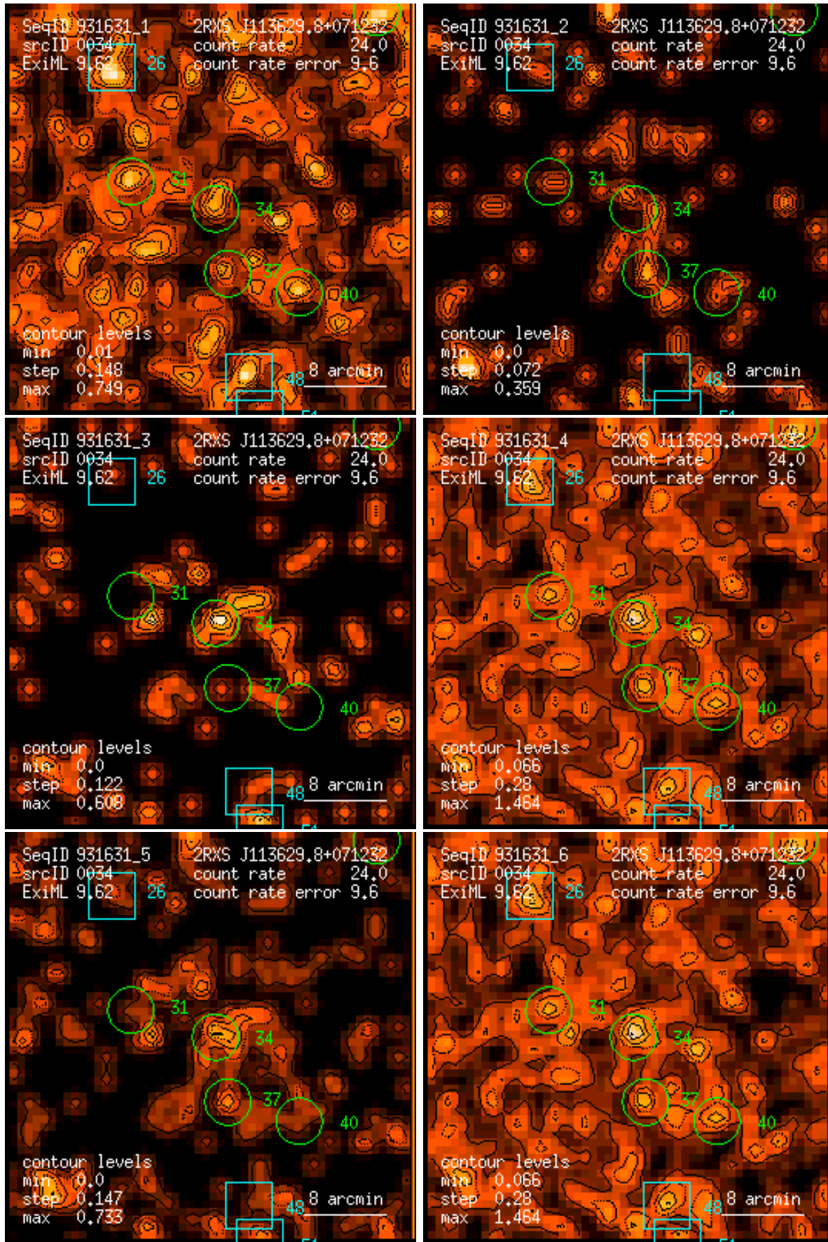
Figure 34: RASS 931631: detection 0034: band rate images, Gaussian filter: (1) PSPC channels 11 – 41, (2) 52 – 90, (3) 91 – 201, (4) 11 – 235, (5) 52 – 201, (6) 11 – 201. Broad band rates in counts/ks. Band rate contour levels in counts/ks/arcmin 2 .
