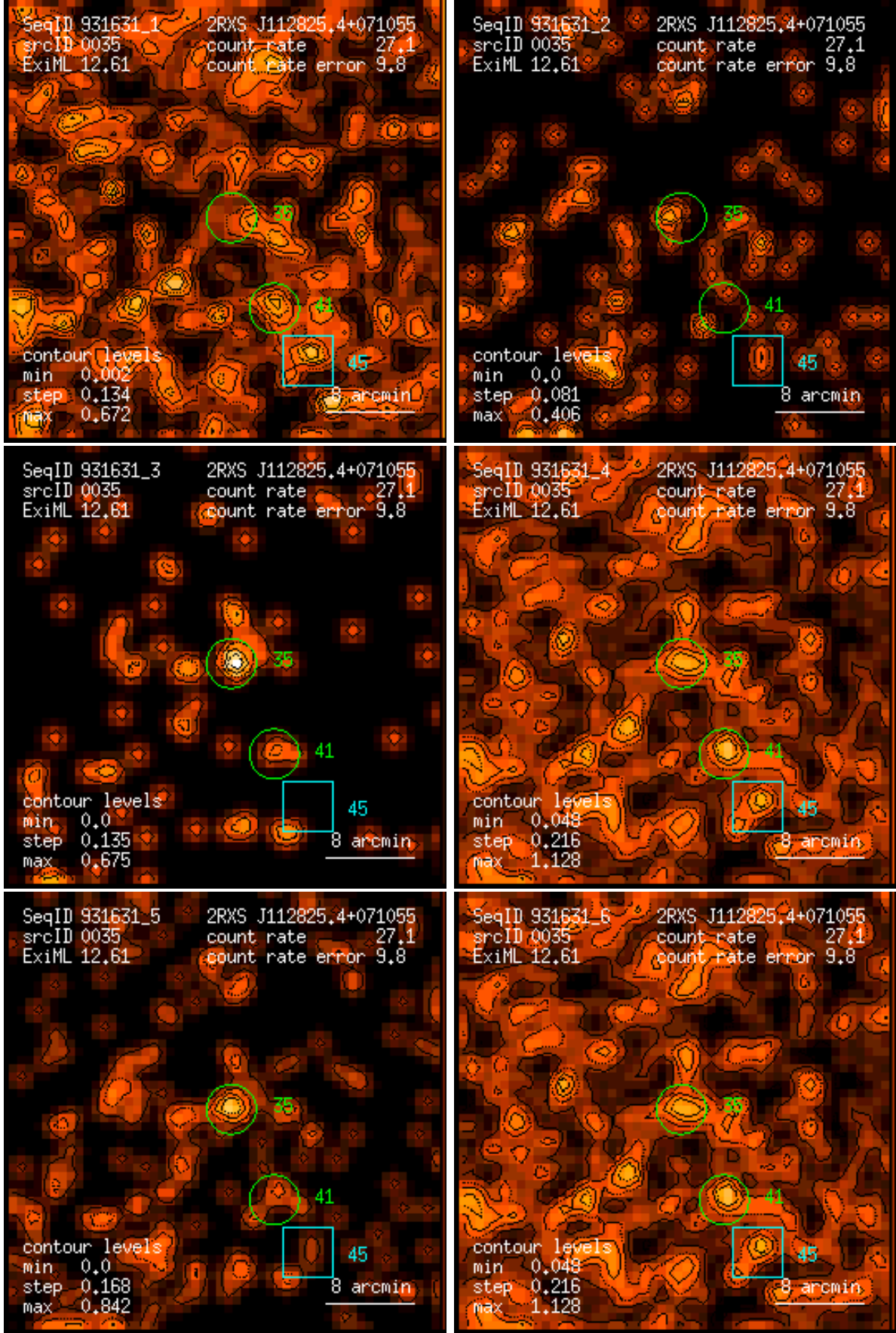
Figure 35: RASS 931631: detection 0035: band rate images, Gaussian filter: (1) PSPC channels 11 – 41, (2) 52 – 90, (3) 91 – 201, (4) 11 – 235, (5) 52 – 201, (6) 11 – 201. Broad band rates in counts/ks. Band rate contour levels in counts/ks/arcmin 2 .
