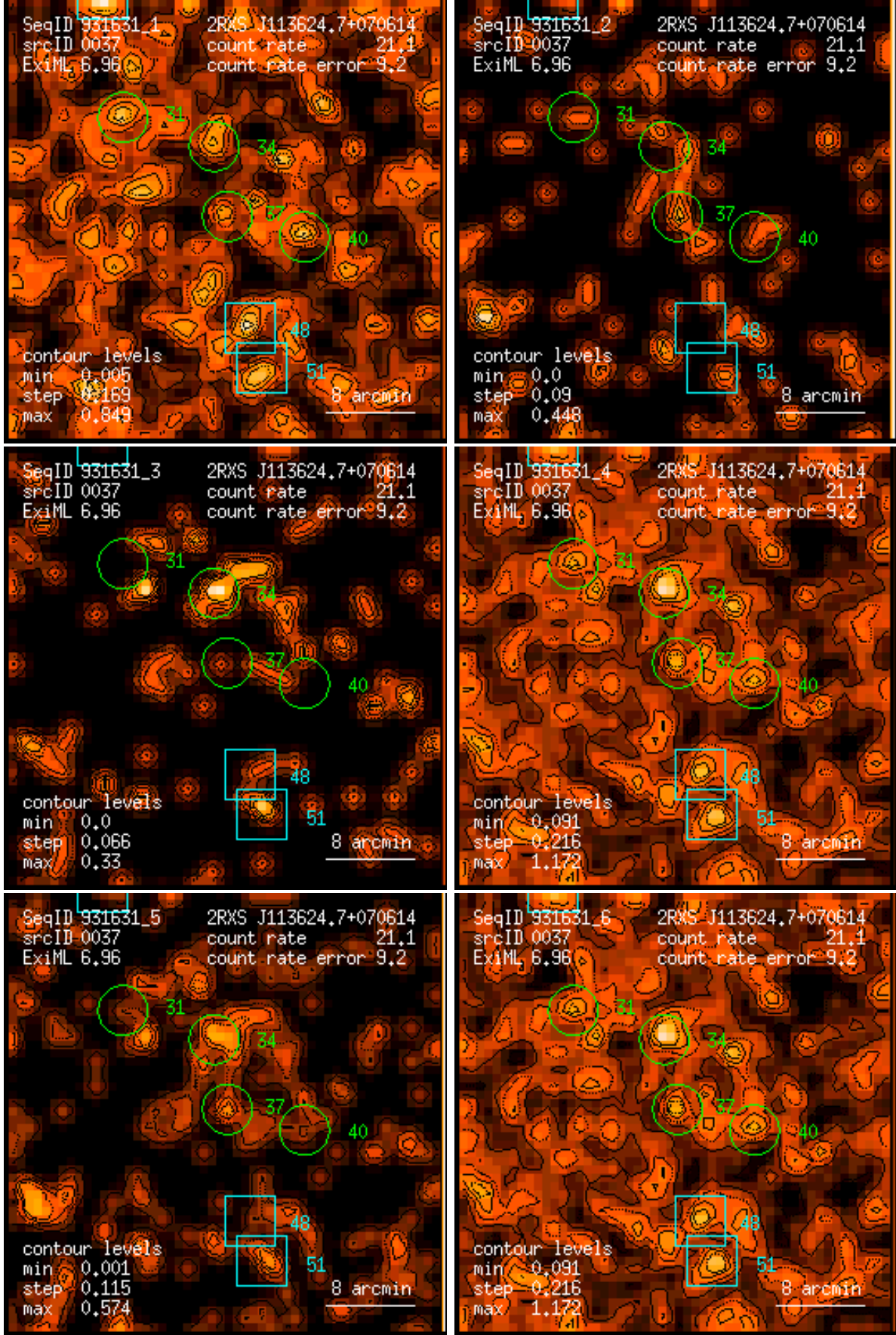
Figure 37: RASS 931631: detection 0037: band rate images, Gaussian filter: (1) PSPC channels 11 – 41, (2) 52 – 90, (3) 91 – 201, (4) 11 – 235, (5) 52 – 201, (6) 11 – 201. Broad band rates in counts/ks. Band rate contour levels in counts/ks/arcmin 2 .
