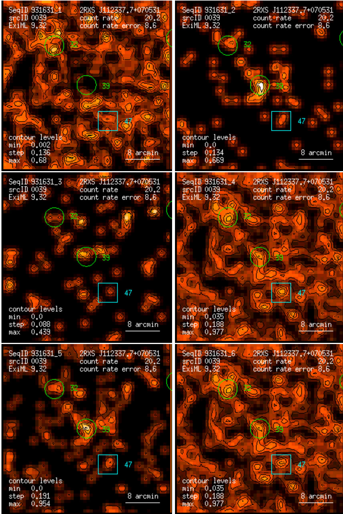
Figure 39: RASS 931631: detection 0039: band rate images, Gaussian filter: (1) PSPC channels 11 – 41, (2) 52 – 90, (3) 91 – 201, (4) 11 – 235, (5) 52 – 201, (6) 11 – 201. Broad band rates in counts/ks. Band rate contour levels in counts/ks/arcmin 2 .
