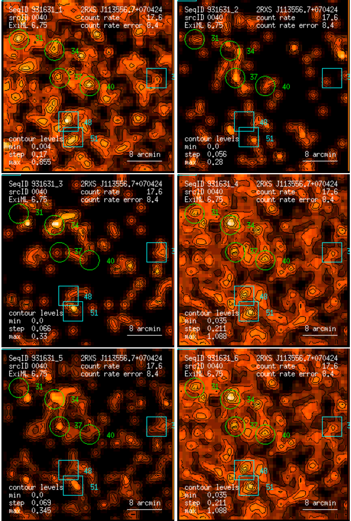
Figure 40: RASS 931631: detection 0040: band rate images, Gaussian filter: (1) PSPC channels 11 – 41, (2) 52 – 90, (3) 91 – 201, (4) 11 – 235, (5) 52 – 201, (6) 11 – 201. Broad band rates in counts/ks. Band rate contour levels in counts/ks/arcmin 2 .
