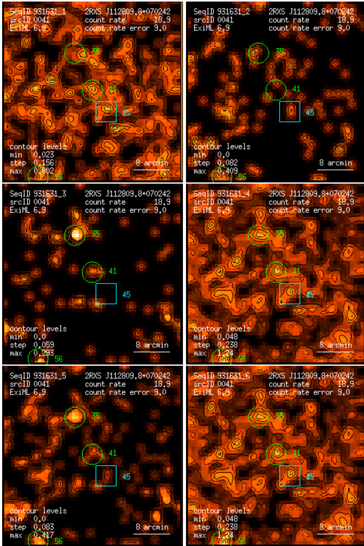
Figure 41: RASS 931631: detection 0041: band rate images, Gaussian filter: (1) PSPC channels 11 – 41, (2) 52 – 90, (3) 91 – 201, (4) 11 – 235, (5) 52 – 201, (6) 11 – 201. Broad band rates in counts/ks. Band rate contour levels in counts/ks/arcmin 2 .
