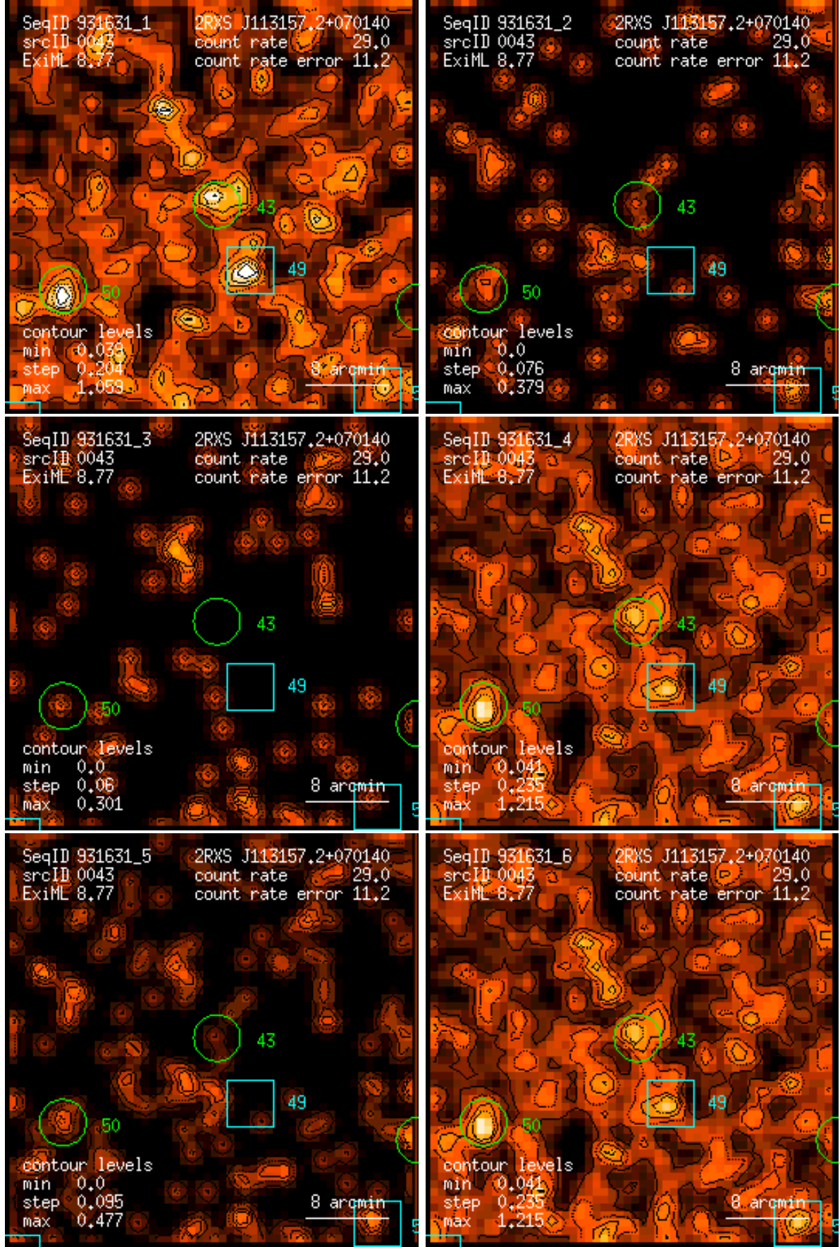
Figure 43: RASS 931631: detection 0043: band rate images, Gaussian filter: (1) PSPC channels 11 – 41, (2) 52 – 90, (3) 91 – 201, (4) 11 – 235, (5) 52 – 201, (6) 11 – 201. Broad band rates in counts/ks. Band rate contour levels in counts/ks/arcmin 2 .
