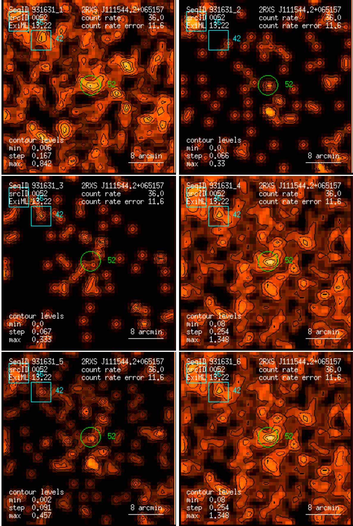
Figure 52: RASS 931631: detection 0052: band rate images, Gaussian filter: (1) PSPC channels 11 – 41, (2) 52 – 90, (3) 91 – 201, (4) 11 – 235, (5) 52 – 201, (6) 11 – 201. Broad band rates in counts/ks. Band rate contour levels in counts/ks/arcmin 2 .
