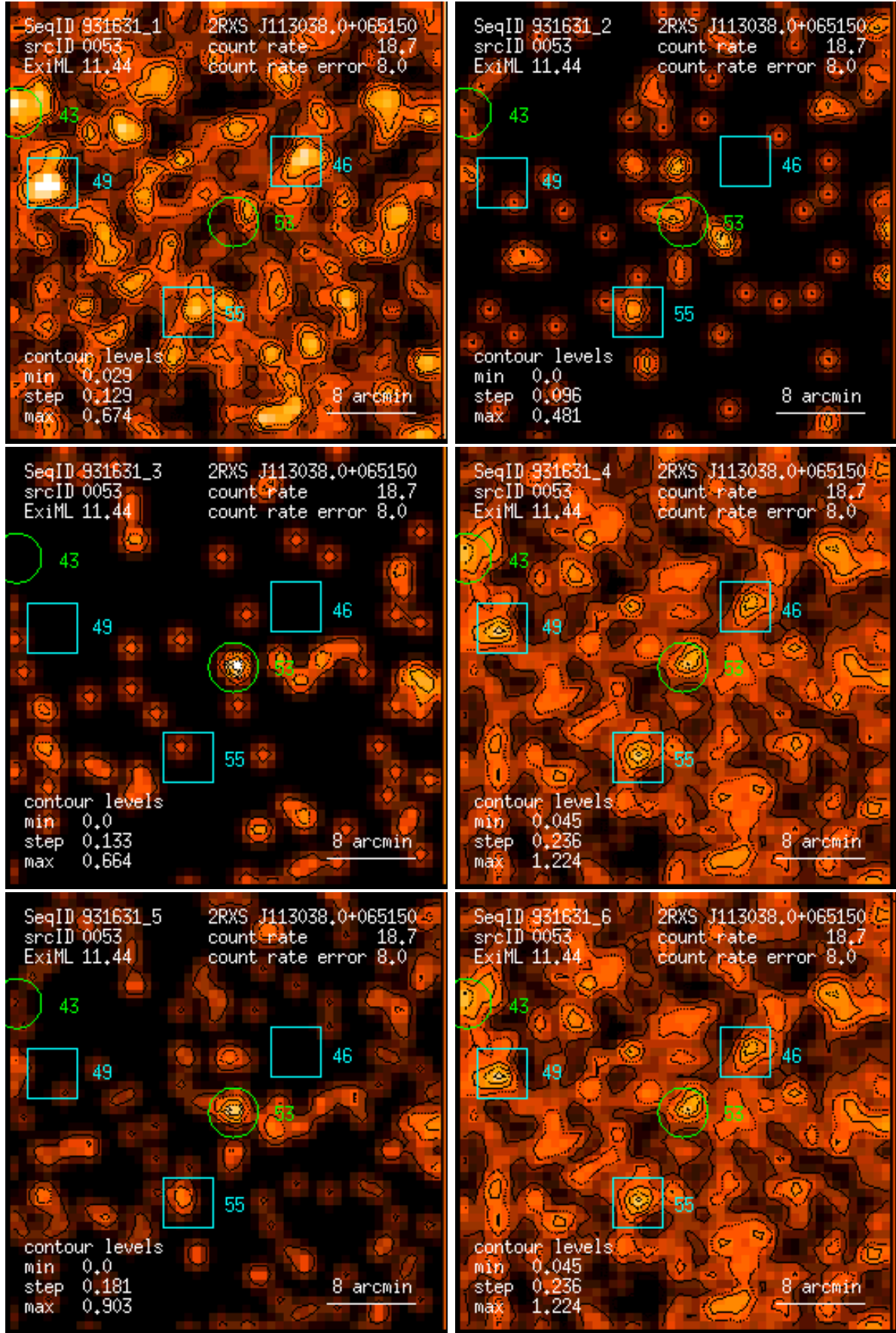
Figure 53: RASS 931631: detection 0053: band rate images, Gaussian filter: (1) PSPC channels 11 – 41, (2) 52 – 90, (3) 91 – 201, (4) 11 – 235, (5) 52 – 201, (6) 11 – 201. Broad band rates in counts/ks. Band rate contour levels in counts/ks/arcmin 2 .
