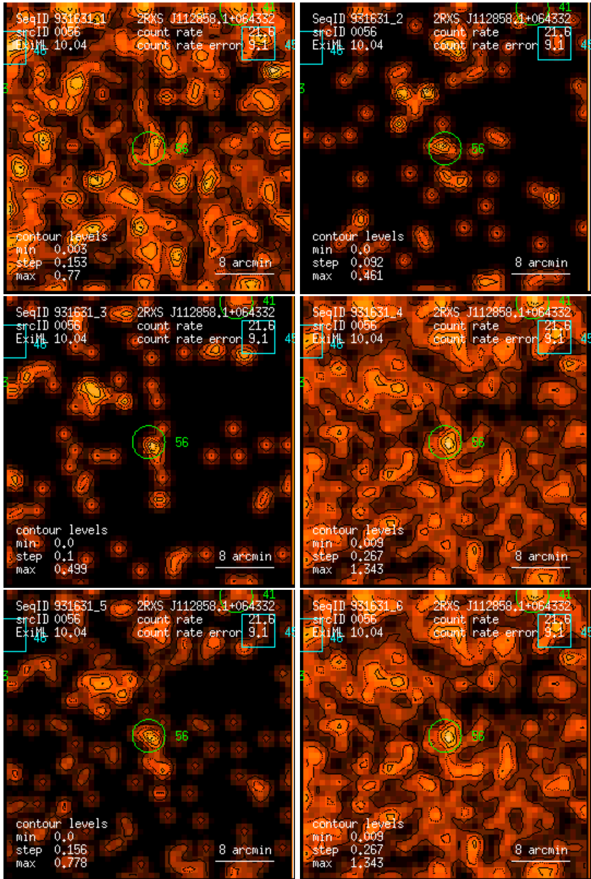
Figure 56: RASS 931631: detection 0056: band rate images, Gaussian filter: (1) PSPC channels 11 – 41, (2) 52 – 90, (3) 91 – 201, (4) 11 – 235, (5) 52 – 201, (6) 11 – 201. Broad band rates in counts/ks. Band rate contour levels in counts/ks/arcmin 2 .
