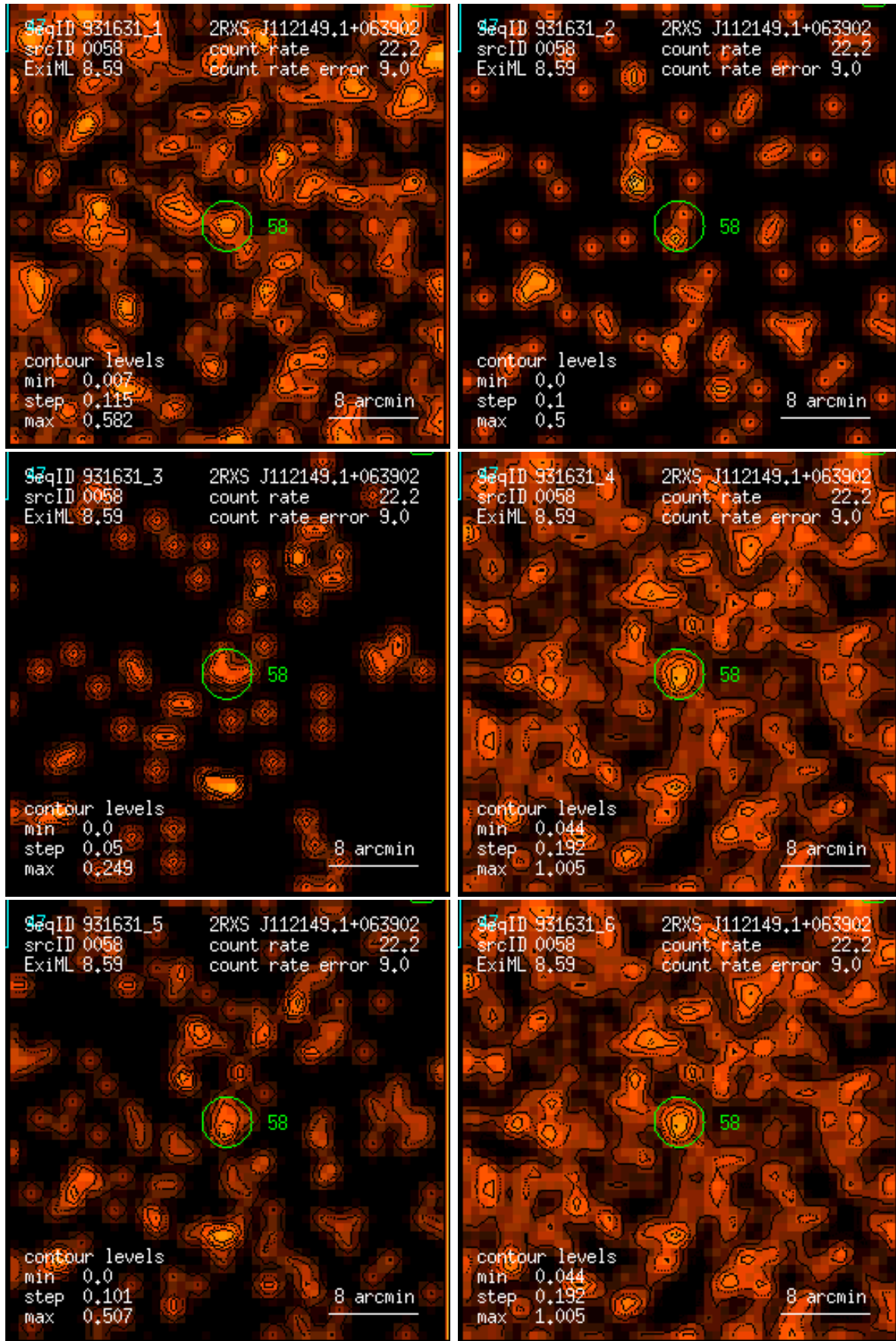
Figure 58: RASS 931631: detection 0058: band rate images, Gaussian filter: (1) PSPC channels 11 – 41, (2) 52 – 90, (3) 91 – 201, (4) 11 – 235, (5) 52 – 201, (6) 11 – 201. Broad band rates in counts/ks. Band rate contour levels in counts/ks/arcmin 2 .
