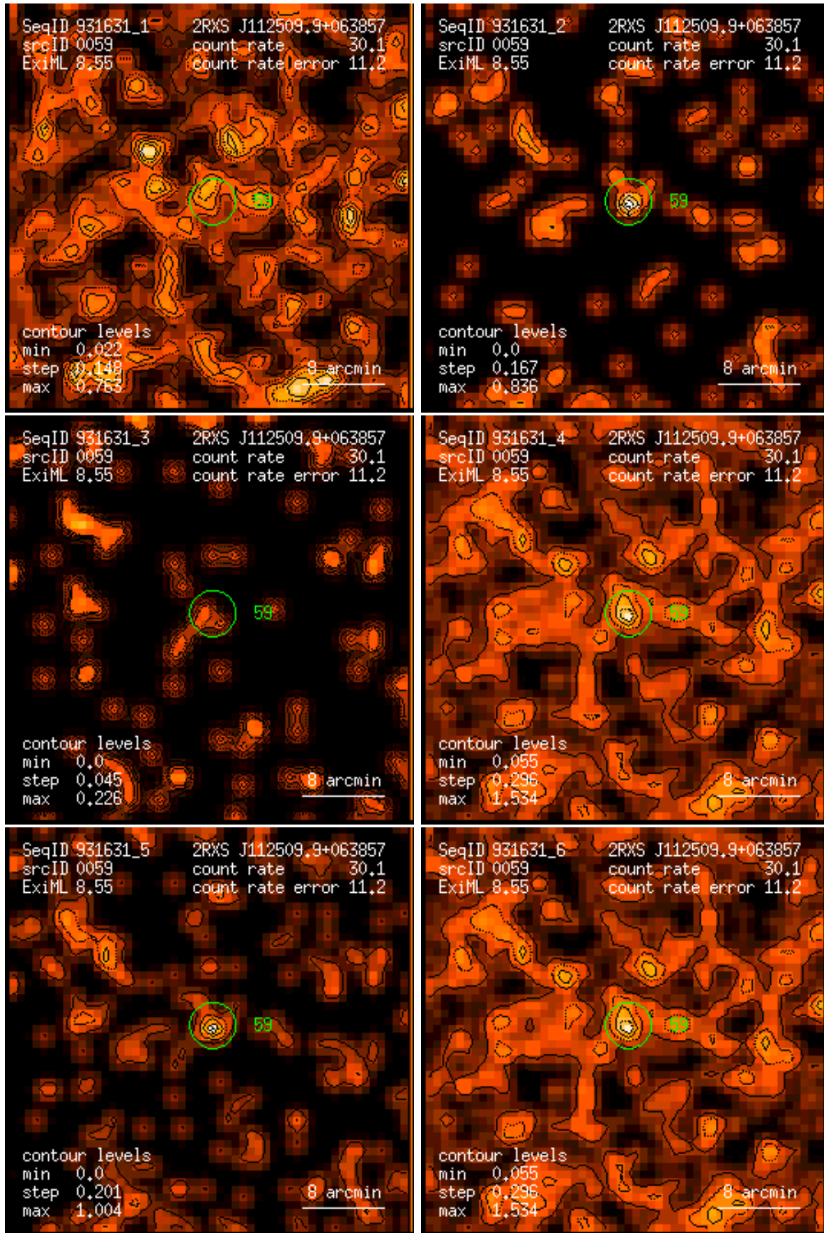
Figure 59: RASS 931631: detection 0059: band rate images, Gaussian filter: (1) PSPC channels 11 – 41, (2) 52 – 90, (3) 91 – 201, (4) 11 – 235, (5) 52 – 201, (6) 11 – 201. Broad band rates in counts/ks. Band rate contour levels in counts/ks/arcmin 2 .
