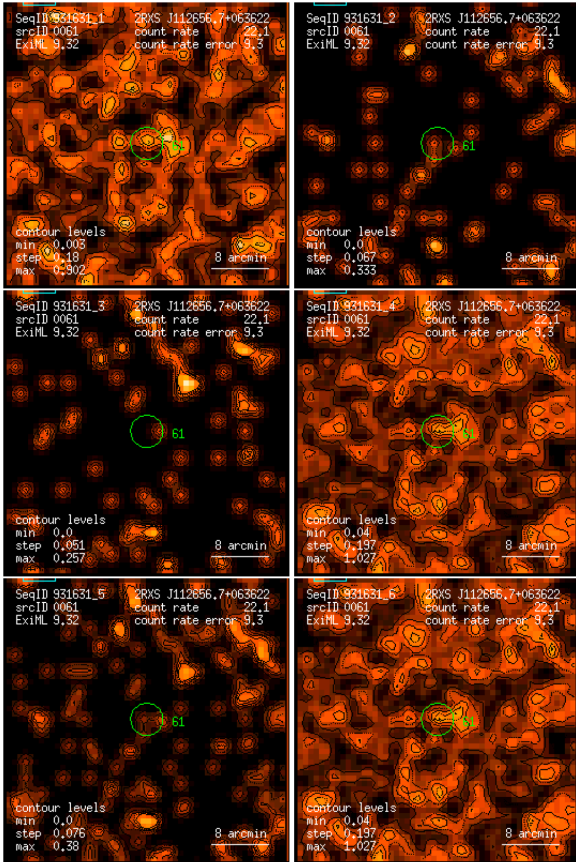
Figure 61: RASS 931631: detection 0061: band rate images, Gaussian filter: (1) PSPC channels 11 – 41, (2) 52 – 90, (3) 91 – 201, (4) 11 – 235, (5) 52 – 201, (6) 11 – 201. Broad band rates in counts/ks. Band rate contour levels in counts/ks/arcmin 2 .
