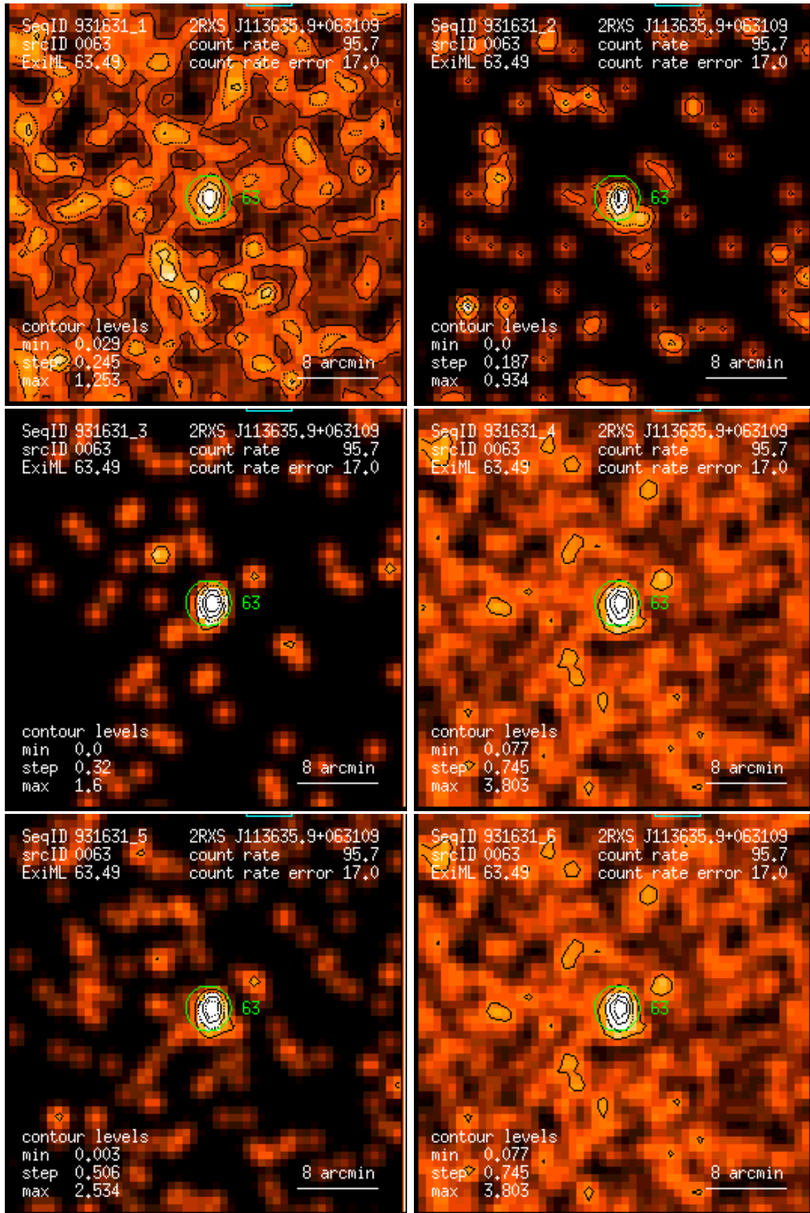
Figure 63: RASS 931631: detection 0063: band rate images, Gaussian filter: (1) PSPC channels 11 – 41, (2) 52 – 90, (3) 91 – 201, (4) 11 – 235, (5) 52 – 201, (6) 11 – 201. Broad band rates in counts/ks. Band rate contour levels in counts/ks/arcmin 2 .
