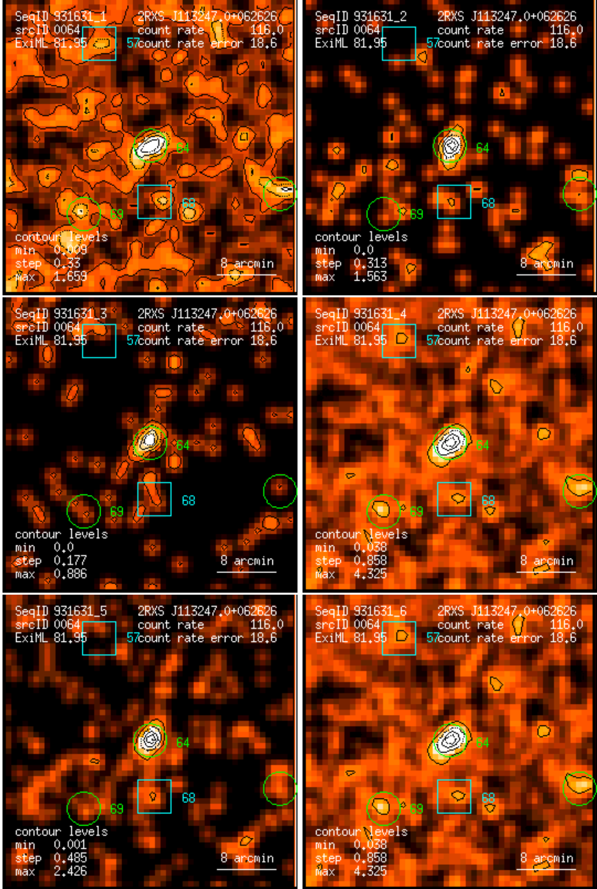
Figure 64: RASS 931631: detection 0064: band rate images, Gaussian filter: (1) PSPC channels 11 – 41, (2) 52 – 90, (3) 91 – 201, (4) 11 – 235, (5) 52 – 201, (6) 11 – 201. Broad band rates in counts/ks. Band rate contour levels in counts/ks/arcmin 2 .
